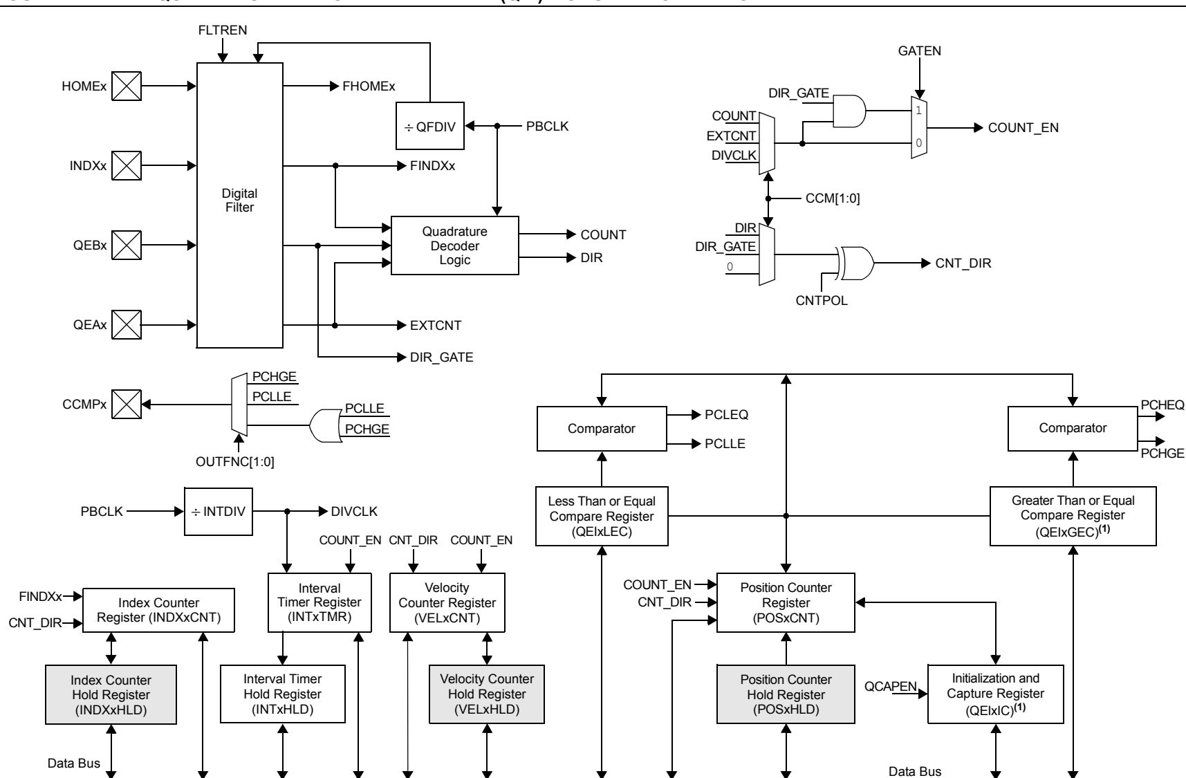
FIGURE 14-2: QUADRATURE ENCODER INTERFACE (QEI) MODULE BLOCK DIAGRAM
