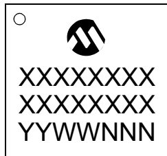
28-Lead UQFN (4x4 mm)
