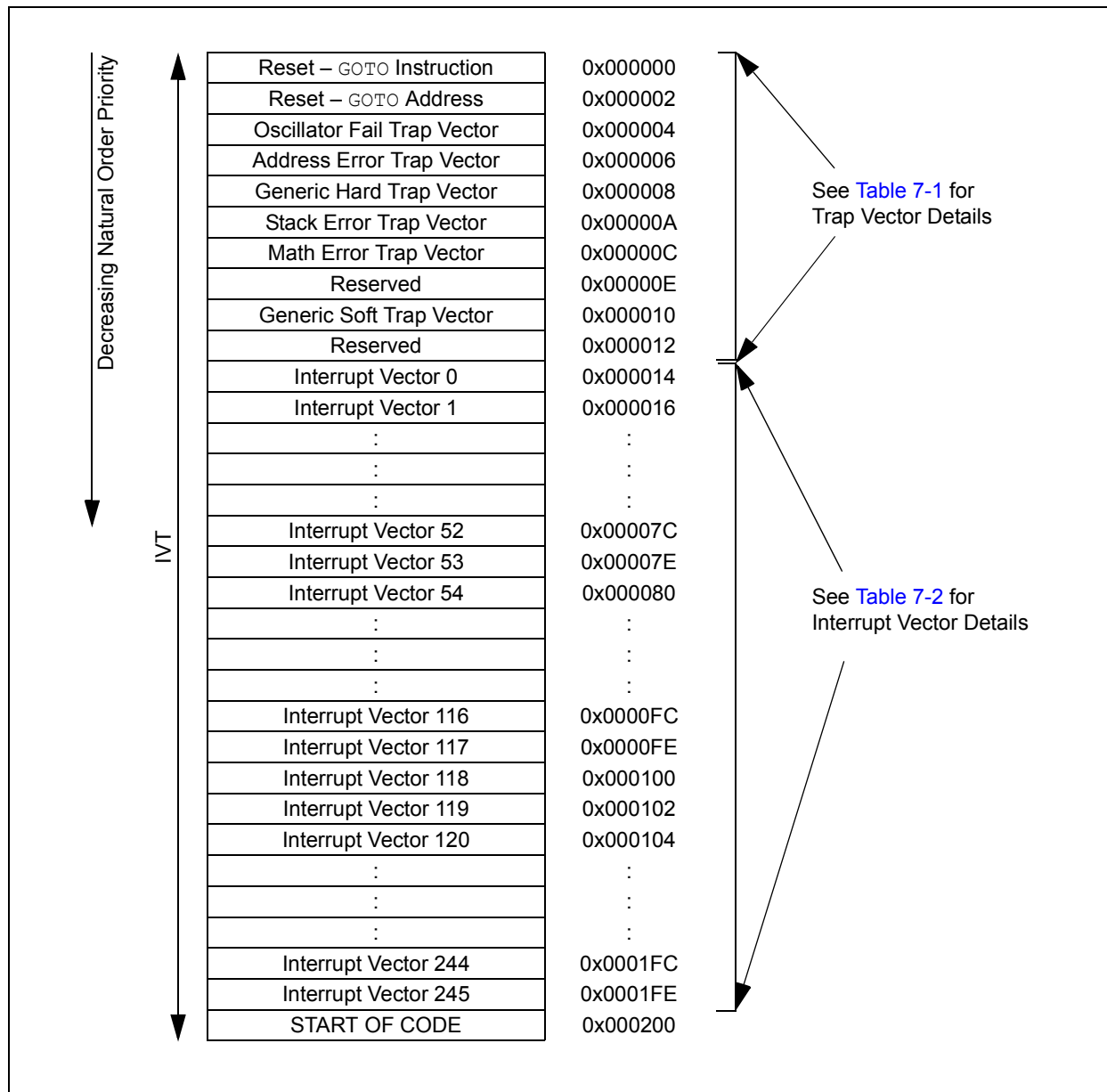
FIGURE 7-1: dsPIC33CK64MP105 FAMILY INTERRUPT VECTOR TABLE
