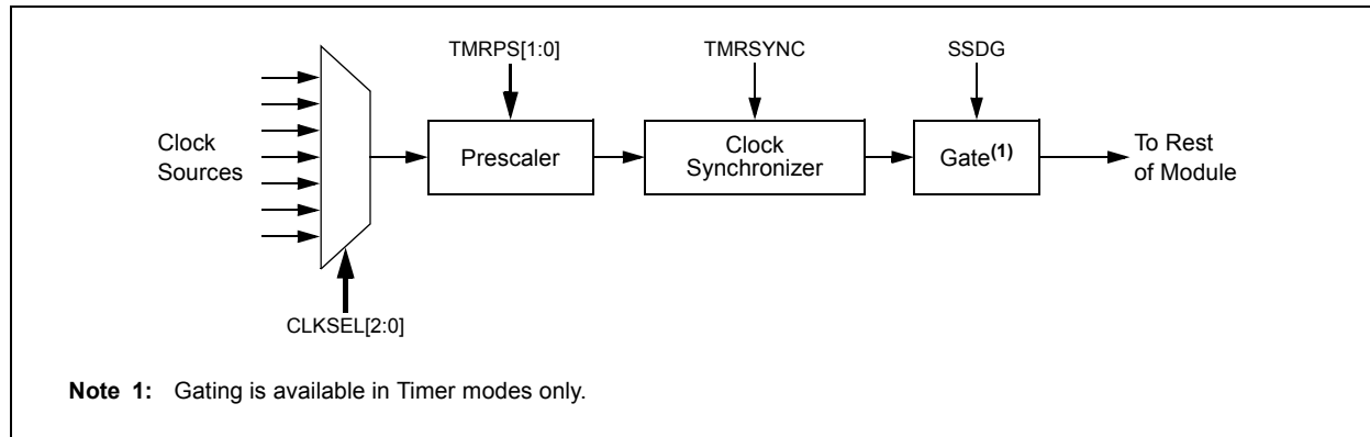
FIGURE 20-2: TIMER CLOCK GENERATOR
