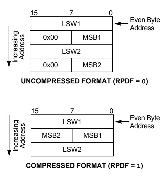
FIGURE 3-15: UNCOMPRESSED/COMPRESSED FORMAT
