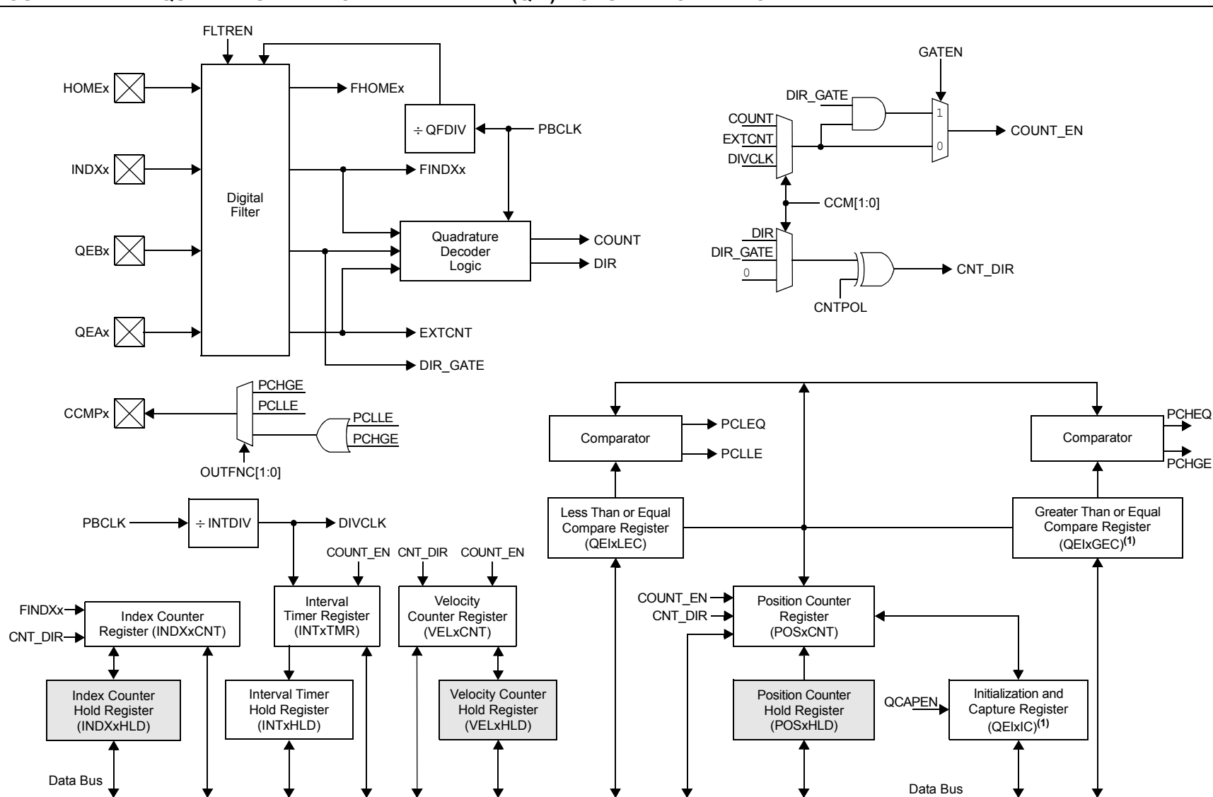
FIGURE 12-2: QUADRATURE ENCODER INTERFACE (QEI) MODULE BLOCK DIAGRAM
