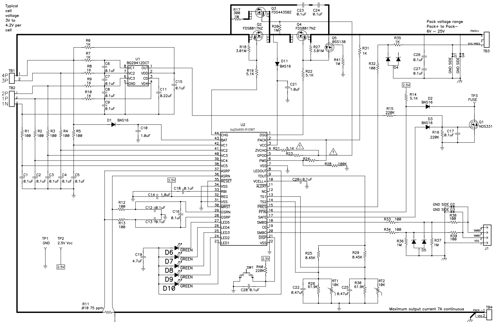
Figure 3. Application Schematic
