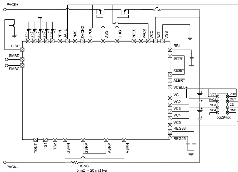
System Partitioning Diagram
