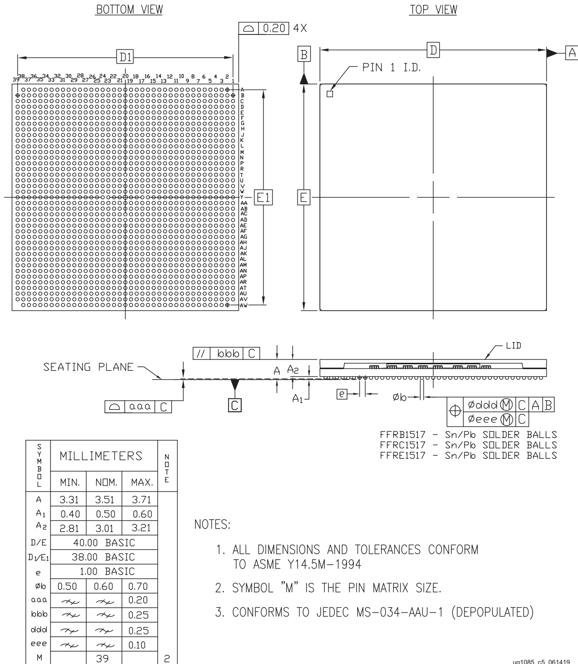
Figure 5-19: Package Dimensions for FFRB1517 (XQZU19EG)
