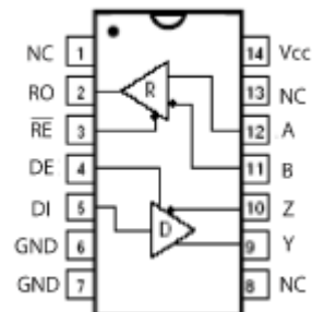
14-Pin PDIP/nSOIC
