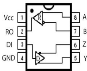
8-Pin PDIP/nSOIC
