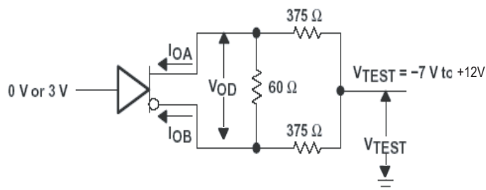
Figure 2. Driver Test Circuit, V_{OD} With Common-Mode Loading
