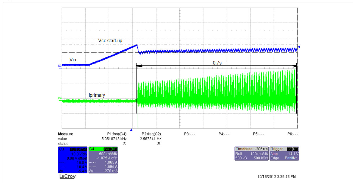
Figure 2.2 ZSLS7031 Soft Start
