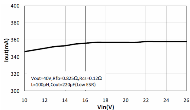
Figure 1.1 V_{IN} vs. I_{OUT} with V_{OUT} = 40V
