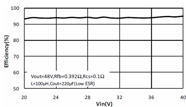
Figure 1.6 V_{IN} vs. Efficiency with V_{OUT} = 48V
