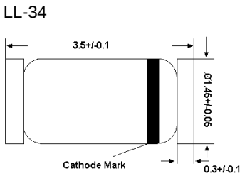
Glass case MiniMELF Dimensions in mm
