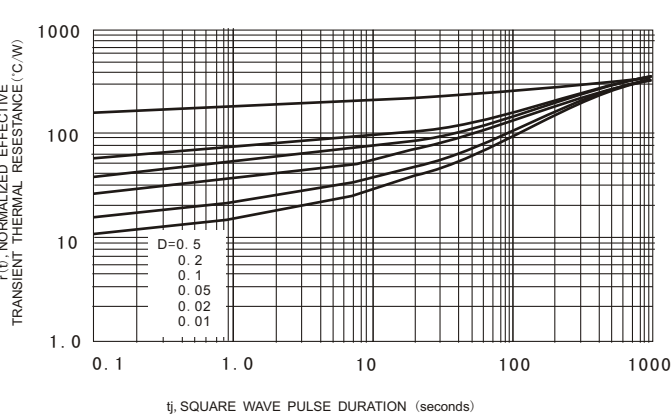
FIG.4-typical Normalized Transient Thermal Impedance Curves
