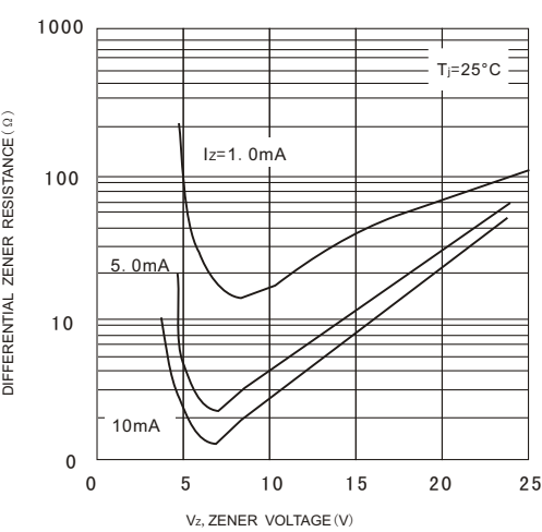
FIG.3-Differential Zener Impedance
