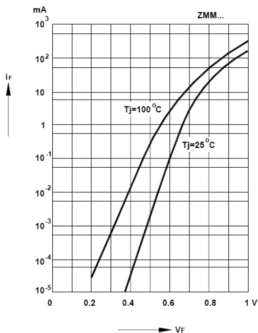
Forward characteristics
