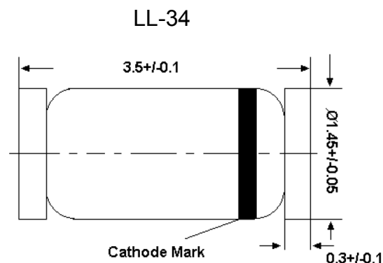
Glass case MiniMELF Dimensions in mm
