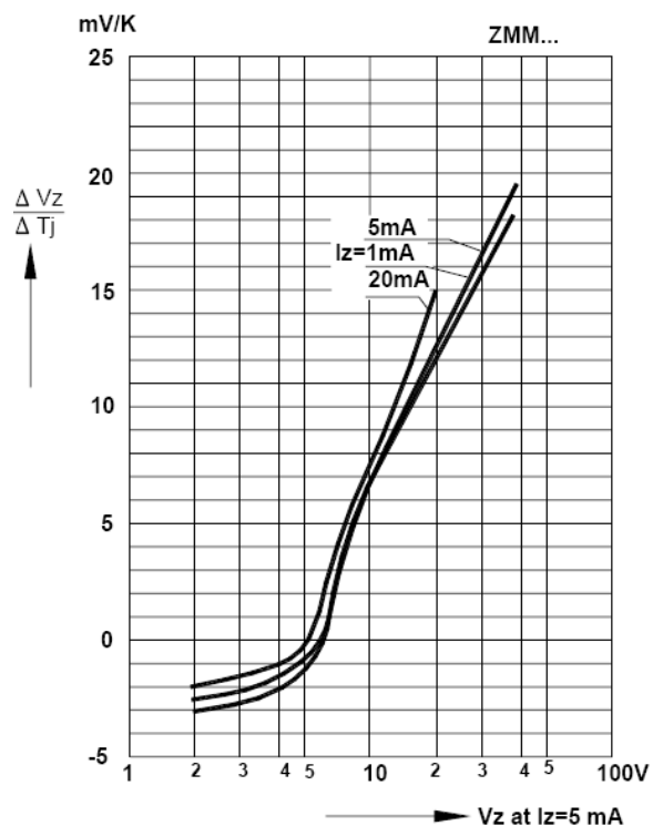
Change of Zener voltage versus junction temperature
