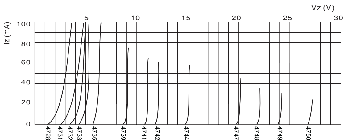
FIG.1 – BREAKDOWN CHARACTERISTICS
