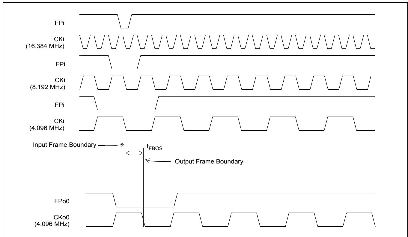
Figure 35 - Input and Output Frame Boundary Offset
