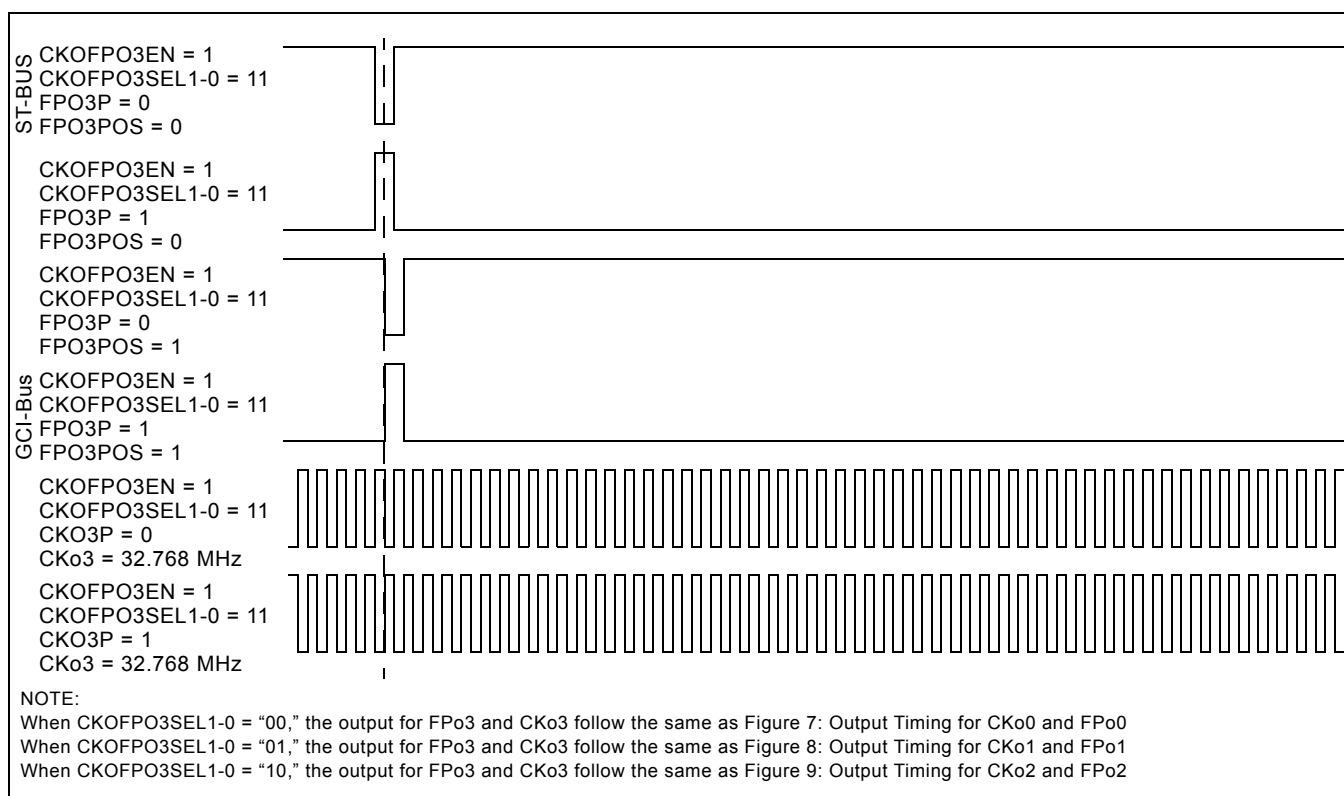
Figure 10 - Output Timing for CKo3 and FPo3 with CKoFPo3SEL1-0="11"
