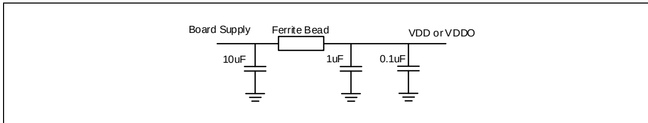
Figure 17. Power Supply Filtering
