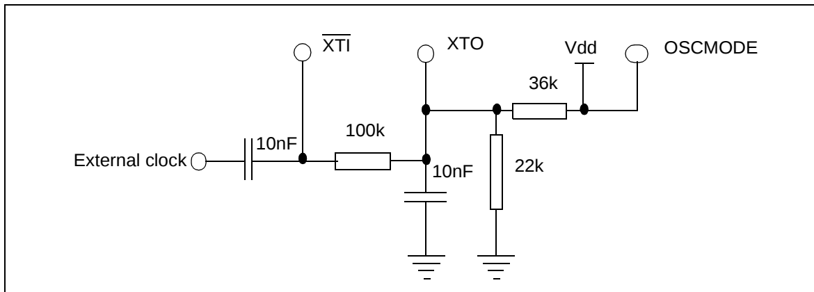
Figure 15 - External Clocking via AC Coupling
