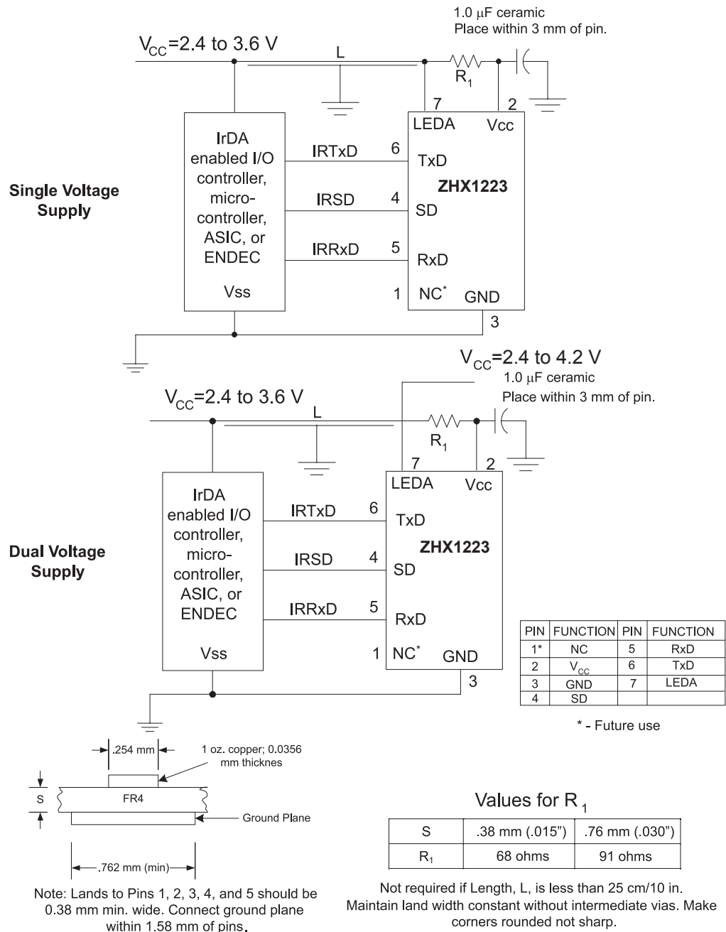
Figure 2. ZHX1223 Application Block Diagrams
