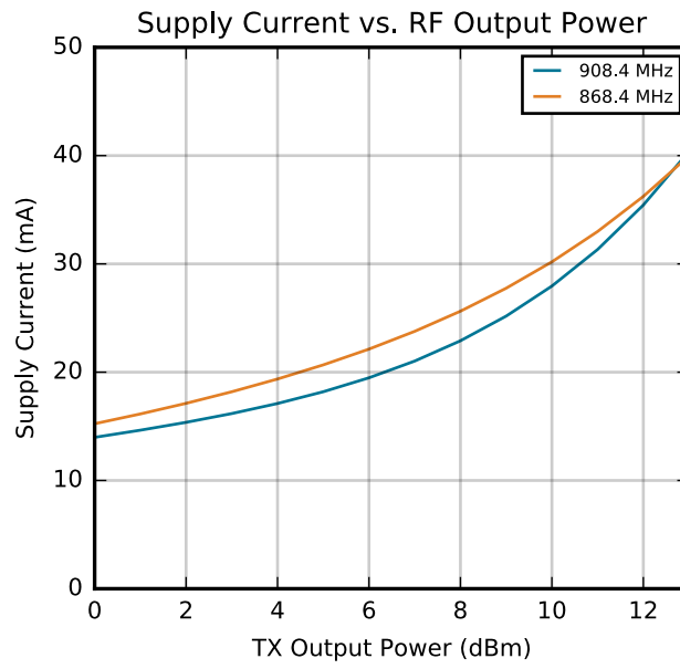
Figure 4.3. RF Transmitter Output Power
