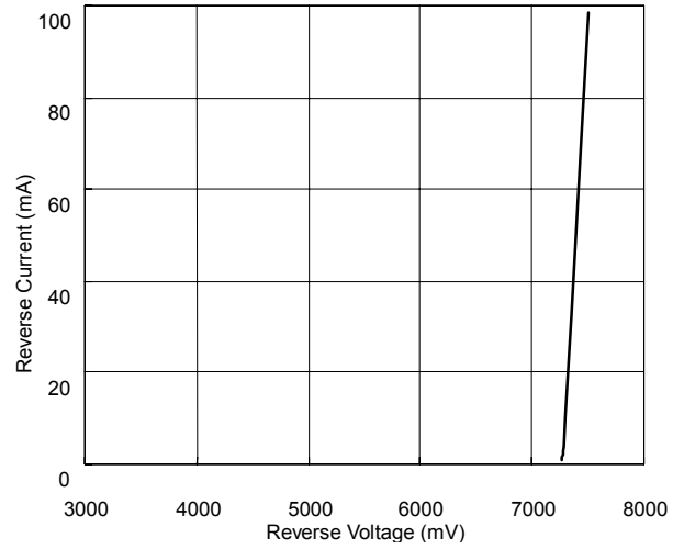
ZD5236A Reverse Current vs Reverse Voltage
