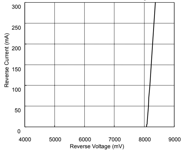
ZD5237A Reverse Current vs Reverse Voltage
