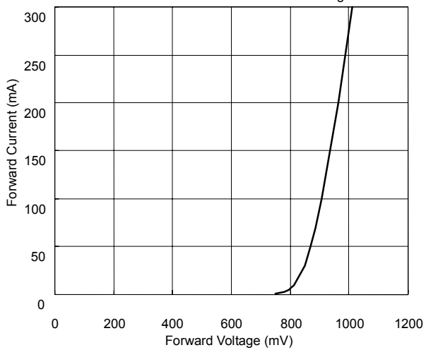
ZD5239A Forward Current vs Forward Voltage
