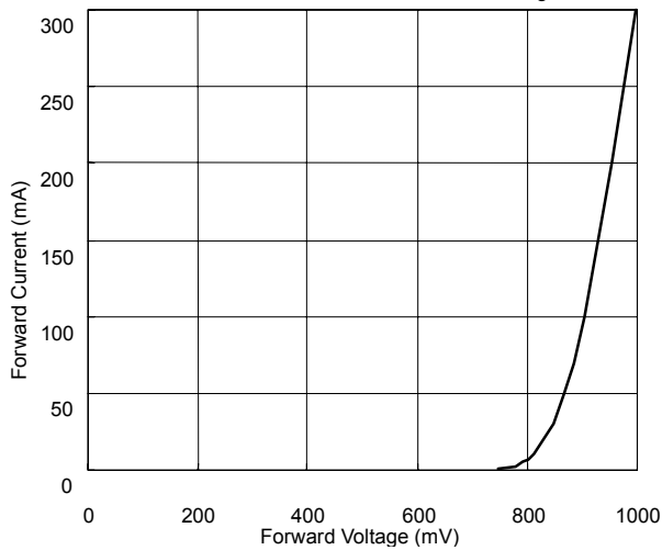
ZD5237A Forward Current vs Forward Voltage
