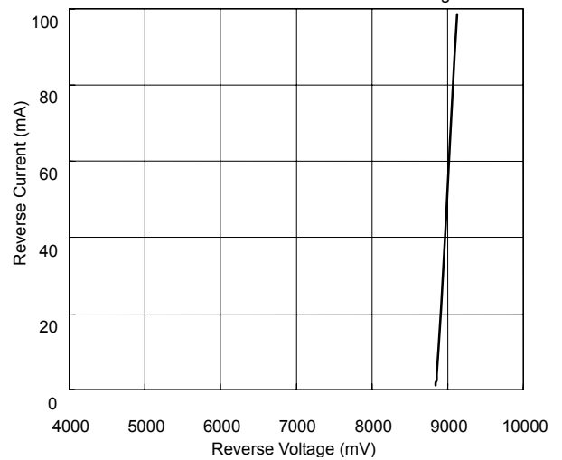
ZD5239A Reverse Current vs Reverse Voltage
