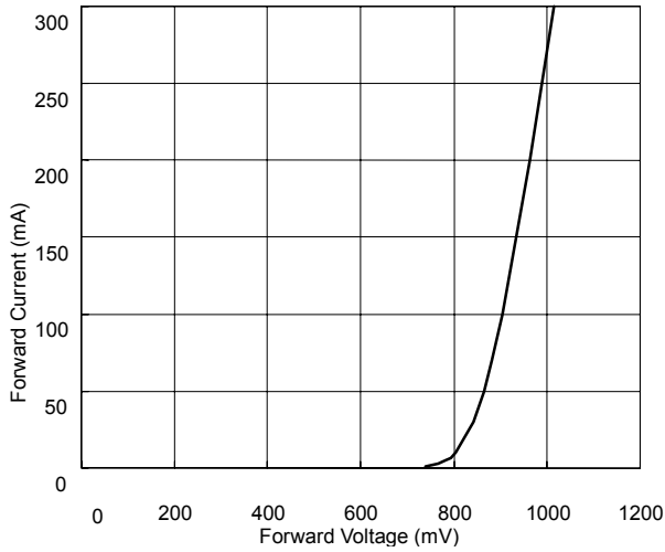
ZD5236A Forward Current vs Forward Voltage
