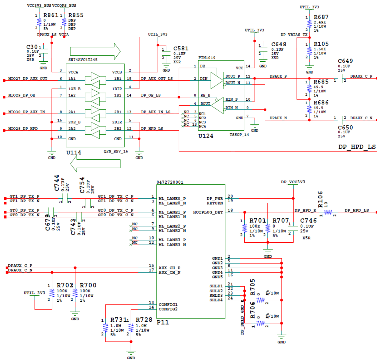
Figure 3-15: DisplayPort Circuit
