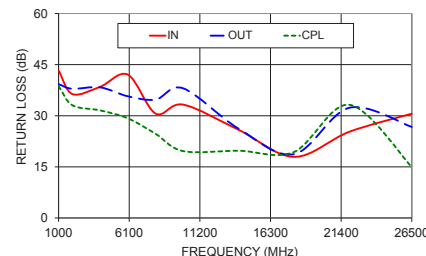
ZCDC10-01263-S+ RETURN LOSS
