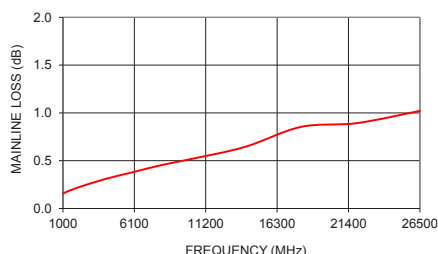
ZCDC10-01263-S+ MAINLINE LOSS
