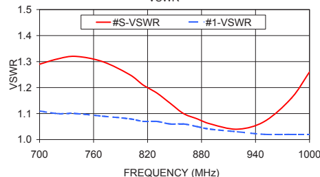
ZC16PD-960W+ VSWR
