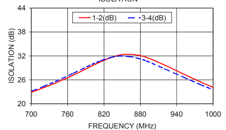
ZC16PD-960W+ ISOLATION
