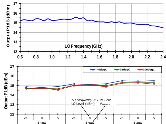
1dB Compression
