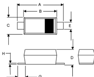
SOD-123
