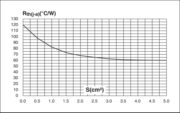
Figure 8. SOT-223 Thermal resistance junction to ambient versus copper surface under tab (printed circuit board FR4, copper thickness: 35 µm)
