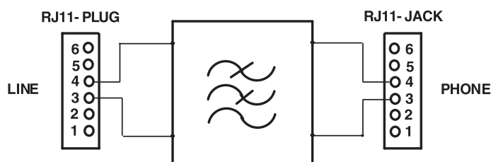
Z-321NF-50 Block Schematic
