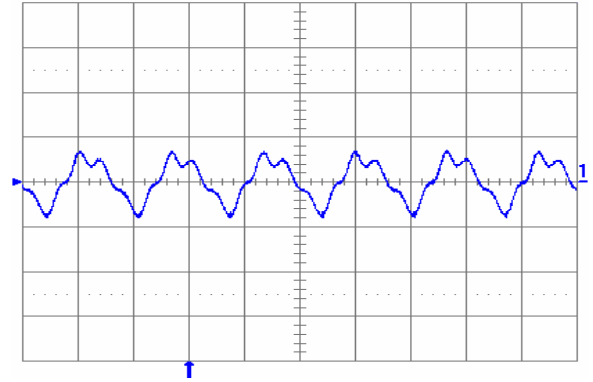
Fig. 3.3V.5: Output voltage ripple (20 mV/div.) at full rated load current into a resistive load with external capacitance 100 \mu F ceramic + 1 \mu F ceramic and V_{in} = 12 V for V_{out} = 3.3 V. Time scale: 2 \mu s/div.
