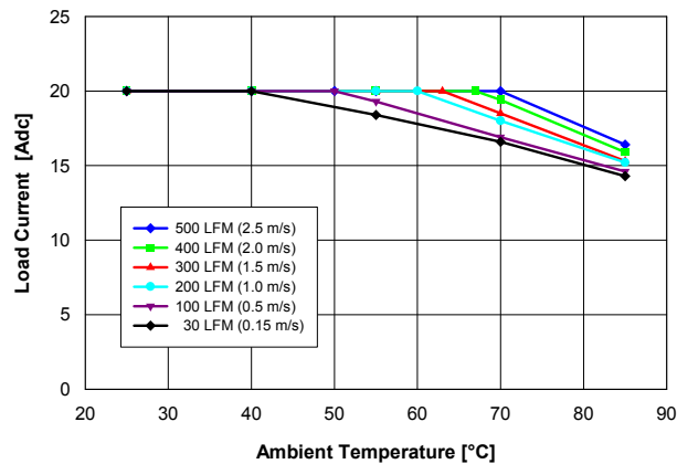
Fig. 1.2V.1: Available load current vs. ambient temperature and airflow rates for V out = 1.2 V converter mounted vertically with V in = 12 V, and maximum MOSFET temperature ≤ 120 °C.
