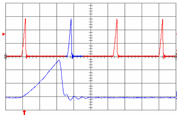
Fig. D: Output short circuit current (10 A/div) ( R_{LOAD} = 10 m \Omega ) for V_{out} = 5.0 V Time scale: 1 ms/div.; Bottom trace: Zoomed current with time scale 0.1 ms/div.
