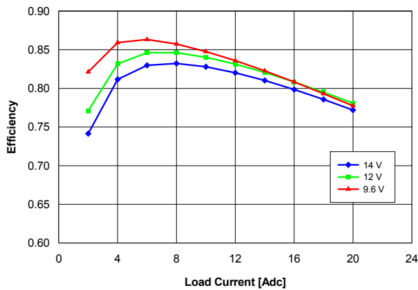
Fig. 1.0V.2: Efficiency vs. load current and input voltage for V out = 1.0 V converter mounted vertically with air flowing at a rate of 200 LFM (1 m/s) and T a = 25 °C.
