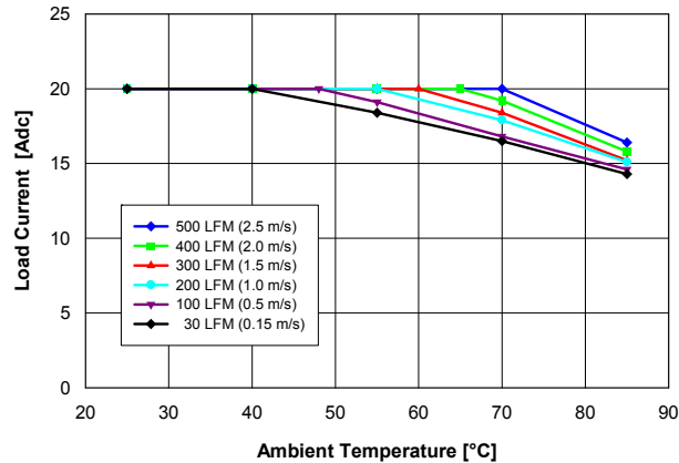
Fig. 1.5V.1: Available load current vs. ambient temperature and airflow rates for V_{out} = 1.5 V converter mounted vertically with V_{in} = 12 V, air flowing and maximum MOSFET temperature \leq 120 °C.
