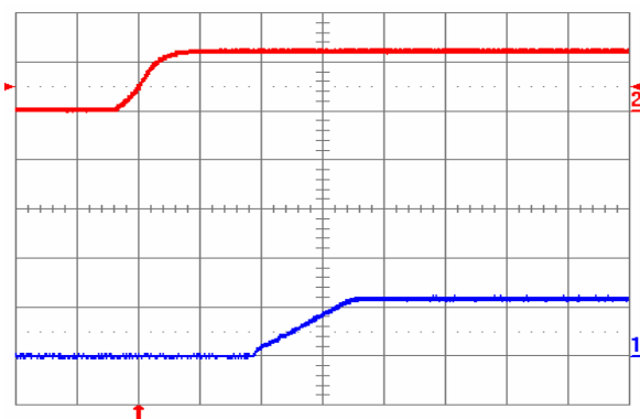
Fig. 1.2V.4: Turn-on transient for V_{out} = 1.2 V with application of V_{in} at full rated load current (resistive) and 100 \mu F external capacitance at V_{in} = 12 V. Top trace: V_{in} (10 V/div.); Bottom trace: output voltage (1 V/div.); Time scale: 2 ms/div.
