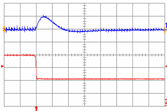
Fig. 1.0V.7: Output voltage response for V_{out} = 1.0 V to negative load current step change from 20 A to 10 A with slew rate of -5A/ \mu s at V_{in} = 12 V. Top trace: output voltage (200 mV/div.); Bottom trace: load current (5 A/div.). C_o = 100 \mu F ceramic. Time scale: 20 \mu s/div.
