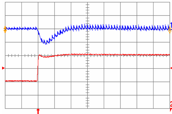
Fig. 1.8V.6: Output voltage response for V_{out} = 1.8 V to positive load current step change from 10 A to 20 A with slew rate of 5 A/ \mu s at V_{in} = 12 V. Top trace: output voltage (200 mV/div.); Bottom trace: load current (5 A/div.). C_o = 100 \mu F ceramic. Time scale: 20 \mu s/div.
