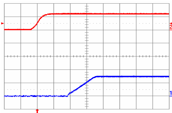
Fig. 1.5V.4: Turn-on transient for V_{out} = 1.5 V with application of V_{in} at full rated load current (resistive) and 100 \mu F external capacitance at V_{in} = 12 V. Top trace: V_{in} (10 V/div.); Bottom trace: output voltage (1 V/div.); Time scale: 2 ms/div.
