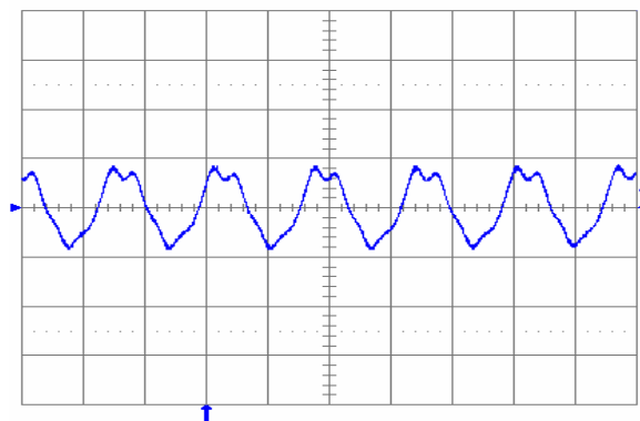
Fig. 5.0V.5: Output voltage ripple (20 mV/div.) at full rated load current into a resistive load with external capacitance 100 \mu F ceramic + 1 \mu F ceramic and V_{in} = 12 V for V_{out} = 5.0 V. Time scale: 2 \mu s/div.
