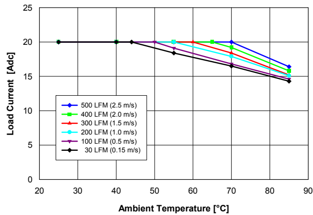
Fig. 1.0V.1: Available load current vs. ambient temperature and airflow rates for V out = 1.0 V converter mounted vertically with V in = 12 V, and maximum MOSFET temperature ≤ 120 °C.
