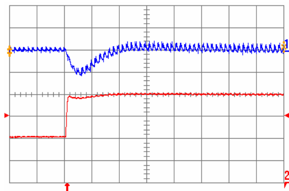
Fig. 2.5V.6: Output voltage response for V_{out} = 2.5 V to positive load current step change from 10 A to 20 A with slew rate of 5 A/ \mu s at V_{in} = 12 V. Top trace: output voltage (200 mV/div.); Bottom trace: load current (5 A/div.). C_o = 100 \mu F ceramic. Time scale: 20 \mu s/div.
