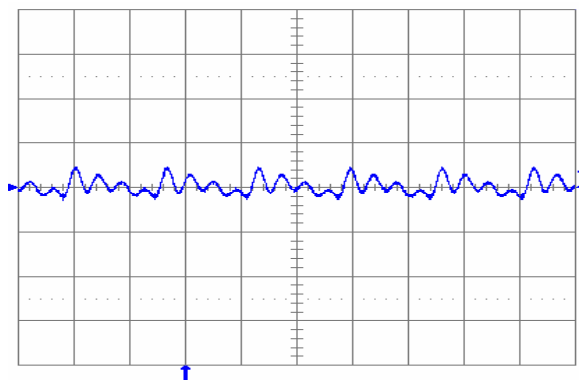
Fig. 1.0V.5: Output voltage ripple (20 mV/div.) at full rated load current into a resistive load with external capacitance 100 \mu F ceramic + 1 \mu F ceramic and V_{in} = 12 V for V_{out} = 1.0 V. Time scale: 2 \mu s/div.
