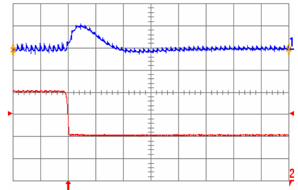
Fig. 1.8V.7: Output voltage response for V_{out} = 1.8 V to negative load current step change from 20 A to 10 A with slew rate of -5 A/ \mu s at V_{in} = 12 V. Top trace: output voltage (200 mV/div.); Bottom trace: load current (5 A/div.). C_o = 100 \mu F ceramic. Time scale: 20 \mu s/div.
