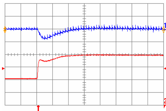
Fig. 0.7525V.6: Output voltage response for V_{out} = 0.7525 V to positive load current step change from 10 A to 20 A with slew rate of 5 A/ \mu s at V_{in} = 12 V. Top trace: output voltage (200 mV/div.); Bottom trace: load current (5 A/div.). C_o = 100 \mu F ceramic. Time scale: 20 \mu s/div.
