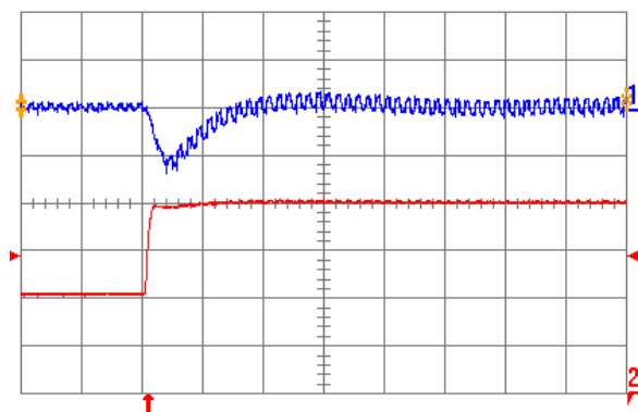
Fig. 5.0V.6: Output voltage response for V_{out} = 5.0 V to positive load current step change from 10 A to 20 A with slew rate of 5 A/ \mu s at V_{in} = 12 V. Top trace: output voltage (200 mV/div.); Bottom trace: load current (5 A/div.). C_o = 100 \mu F ceramic. Time scale: 20 \mu s/div.
