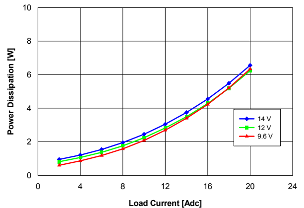
Fig. 3.3V.3: Power loss vs. load current and input voltage for V_{out} = 3.3 V converter mounted vertically with air flowing at a rate of 200 LFM (1 m/s) and T_a = 25 °C.
