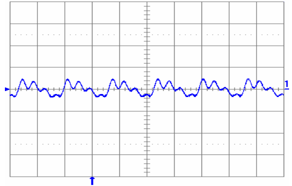
Fig. 1.8V.5: Output voltage ripple (20 mV/div.) at full rated load current into a resistive load with external capacitance 100 \mu F ceramic + 1 \mu F ceramic and V_{in} = 12 V for V_{out} = 1.8 V. Time scale: 2 \mu s/div.
