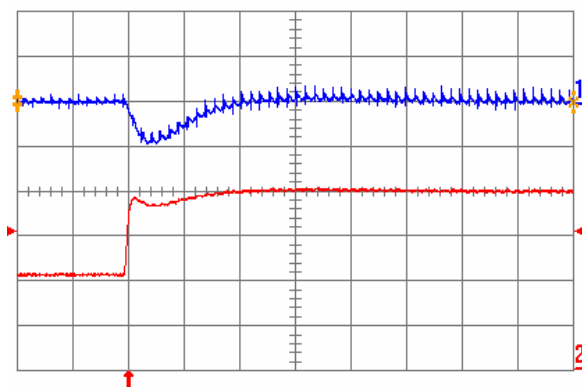
Fig. 1.0V.6: Output voltage response for V_{out} = 1.0 V to positive load current step change from 10 A to 20 A with slew rate of 5A/ \mu s at V_{in} = 12 V. Top trace: output voltage (200 mV/div.); Bottom trace: load current (5 A/div.). C_o = 100 \mu F ceramic. Time scale: 20 \mu s/div.
