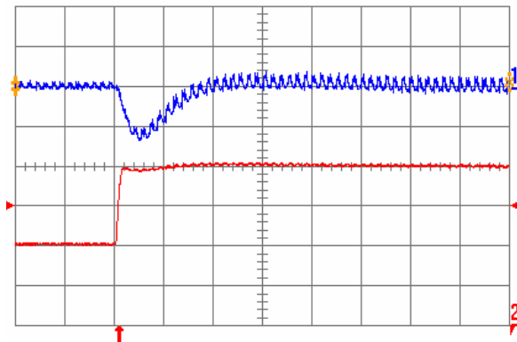
Fig. 3.3V.6: Output voltage response for V_{out} = 3.3 V to positive load current step change from 10 A to 20 A with slew rate of 5 A/ \mu s at V_{in} = 12 V. Top trace: output voltage (200 mV/div.); Bottom trace: load current (5 A/div.). C_o = 100 \mu F ceramic. Time scale: 20 \mu s/div.
