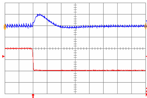
Fig. 1.5V.7: Output voltage response for V_{out} = 1.5 V to negative load current step change from 20 A to 10 A with slew rate of -5 A/ \mu s at V_{in} = 12 V. Top trace: output voltage (200 mV/div.); Bottom trace: load current (5 A/div.). C_o = 100 \mu F ceramic. Time scale: 20 \mu s/div.
