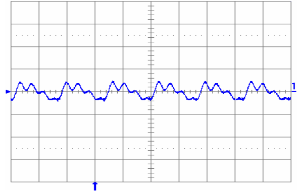
Fig. 2.0V.5: Output voltage ripple (20 mV/div.) at full rated load current into a resistive load with external capacitance 100 \mu\text{F} ceramic + 1 \mu\text{F} ceramic and V_{in} = 12 V for V_{out} = 2.0 V. Time scale: 2 \mu\text{s} /div.
