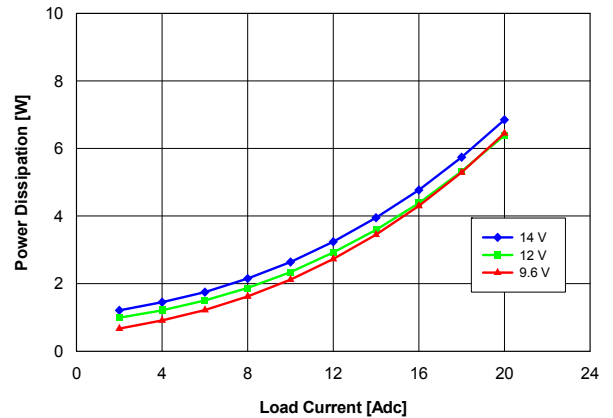
Fig. 5.0V.3: Power loss vs. load current and input voltage for V_{out} = 5.0 V converter mounted vertically with air flowing at a rate of 200 LFM (1 m/s) and T_a = 25 °C.
