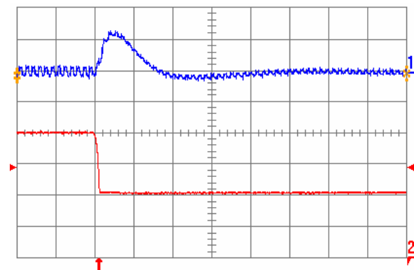
Fig. 5.0V.7: Output voltage response for V_{out} = 5.0 V to negative load current step change from 20 A to 10 A with slew rate of -5 A/ \mu s at V_{in} = 12 V. Top trace: output voltage (200 mV/div.); Bottom trace: load current (5 A/div.). C_o = 100 \mu F ceramic. Time scale: 20 \mu s/div.
