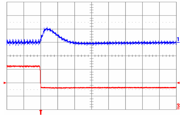
Fig. 2.0V.7: Output voltage response for V_{out} = 2.0 V to negative load current step change from 20 A to 10 A with slew rate of -5 \text{ A}/\mu\text{s} at V_{in} = 12 V. Top trace: output voltage (200 mV/div.); Bottom trace: load current (5 A/div.). C_o = 100 \mu\text{F} ceramic. Time scale: 20 \mu\text{s} /div.
