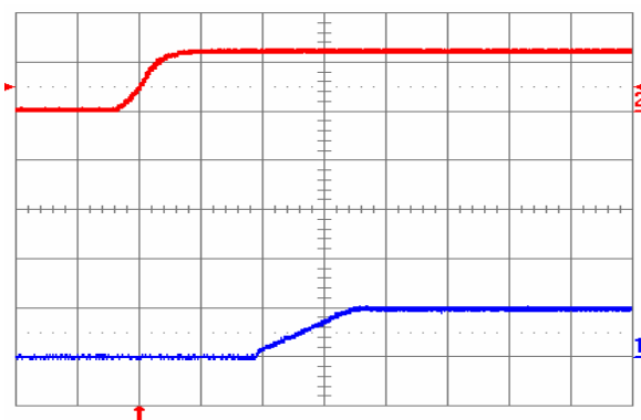
Fig. 1.0V.4: Turn-on transient for V_{out} = 1.0 V with application of V_{in} at full rated load current (resistive) and 100 \mu F external capacitance at V_{in} = 12 V. Top trace: V_{in} (10 V/div.); Bottom trace: output voltage (1 V/div.); Time scale: 2 ms/div.
