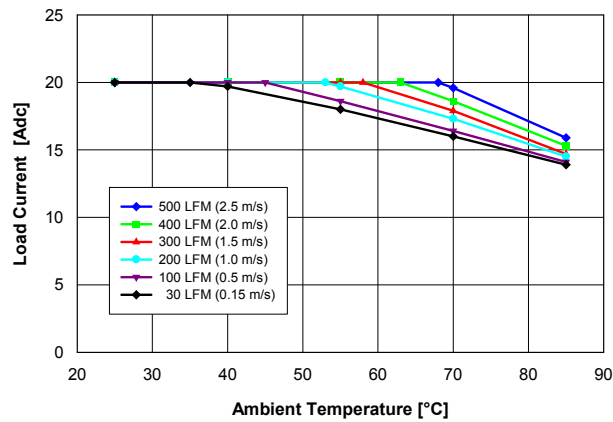
Fig. 2.0V.1: Available load current vs. ambient temperature and airflow rates for V out = 2.0 V converter mounted vertically with V in = 12 V, and maximum MOSFET temperature ≤ 120 °C.
