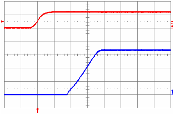
Fig. 3.3V.4: Turn-on transient for V_{out} = 3.3 V with application of V_{in} at full rated load current (resistive) and 100 \mu F external capacitance at V_{in} = 12 V. Top trace: V_{in} (10 V/div.); Bottom trace: output voltage (1 V/div.); Time scale: 2 ms/div.
