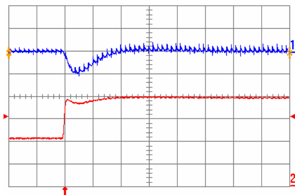
Fig. 1.2V.6: Output voltage response for V_{out} = 1.2 V to positive load current step change from 10 A to 20 A with slew rate of 5 A/ \mu s at V_{in} = 12 V. Top trace: output voltage (200 mV/div.); Bottom trace: load current (5 A/div.). C_o = 100 \mu F ceramic. Time scale: 20 \mu s/div.
