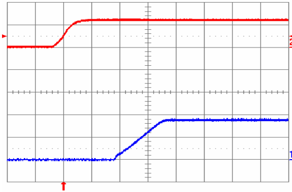
Fig. 1.8V.4: Turn-on transient for V_{out} = 1.8 V with application of V_{in} at full rated load current (resistive) and 100 \mu F external capacitance at V_{in} = 12 V. Top trace: V_{in} (10 V/div.); Bottom trace: output voltage (1 V/div.); Time scale: 2 ms/div.
