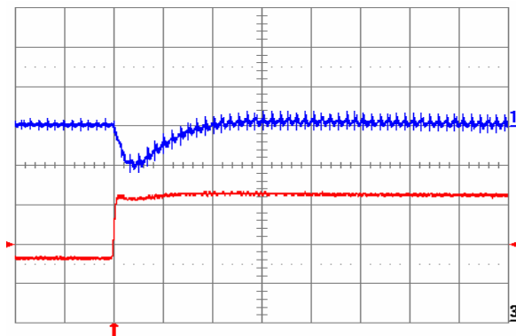
Fig. 2.0V.6: Output voltage response for V_{out} = 2.0 V to positive load current step change from 10 A to 20 A with slew rate of 5 \text{ A}/\mu\text{s} at V_{in} = 12 V. Top trace: output voltage (200 mV/div.); Bottom trace: load current (5 A/div.). C_o = 100 \mu\text{F} ceramic. Time scale: 20 \mu\text{s} /div.
