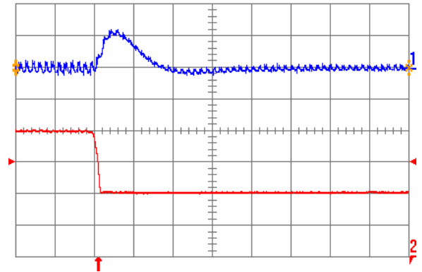
Fig. 3.3V.7: Output voltage response for V_{out} = 3.3 V to negative load current step change from 20 A to 10 A with slew rate of -5A/ \mu s at V_{in} = 12 V. Top trace: output voltage (200 mV/div.); Bottom trace: load current (5 A/div.). C_o = 100 \mu F ceramic. Time scale: 20 \mu s/div.
