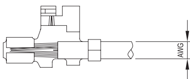
AWG: #22~#28
