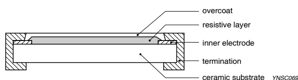
Fig. 3 Chip resistor outlines
