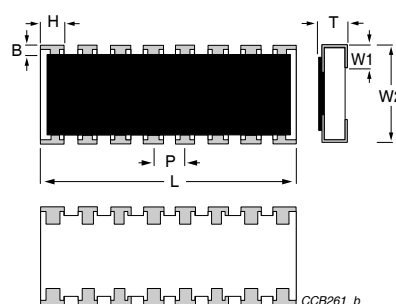
Fig. 4 YC248 series chip resistors dimension
