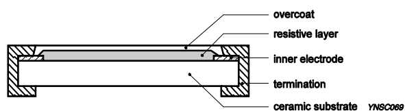
Fig. 9 Chip resistor outlines
