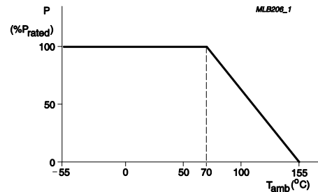
Fig. 12 Maximum dissipation (P) in percentage of rated power as a function of the operating ambient temperature ( T_{amb} )
