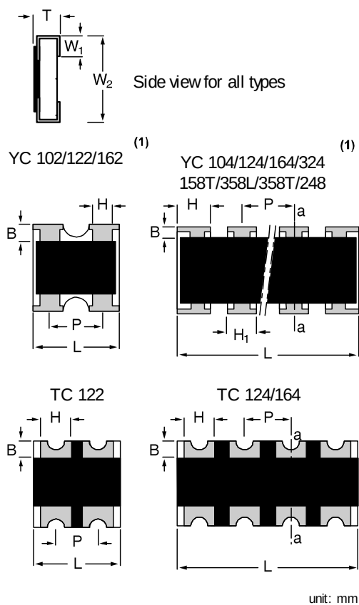
Fig. 12 YC/TC122 series chip resistors dimension Note: (1) YC102/104 is flat type
