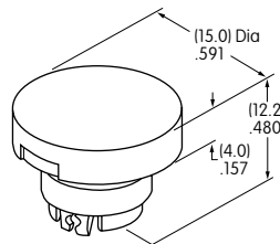
AT3002 Round
