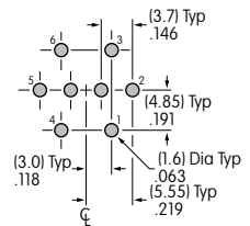
Double Pole
