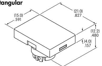
AT3003 Rectangular
