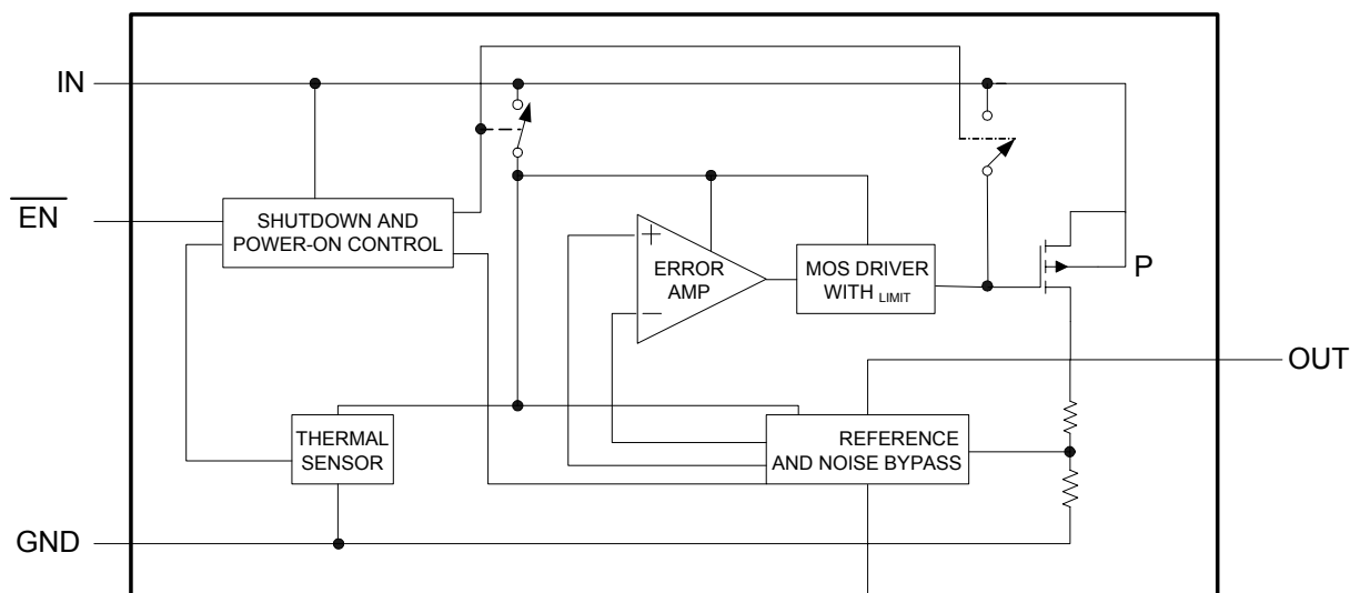
Figure 3. Block Diagram
