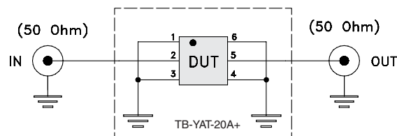
Fig 1. Block diagram of Test Circuit used for characterization, Test board TB-YAT-20A+ Conditions: Attenuation, VSWR: Pin=-10 dBm
