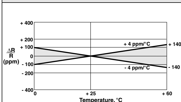
FIGURE 3 - TEMPERATURE COEFFICIENT
