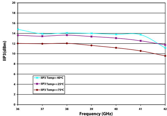
LSB IIP3 for XU1006-QB Vg2=-0.5V, Vd=4V, Id=240mA, P_LO=+4dBm, P_IF/100Hz=-5dBm, F=10 MHz
