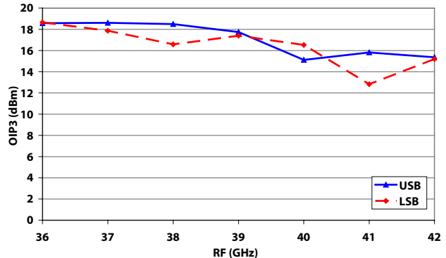
XU1006-QB, Output IP3 (dBm)
