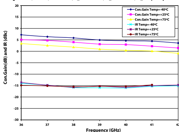
USB Conversion Gain (dB) and IR (dBc) for XU1006-QB Vg2=-0.5V, Vd=4V, Id=240mA, P_LO=+4dBm, P_IF=-10dBm, IF_Frequency=2 GHz
