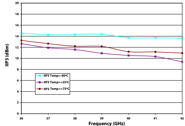
USB IIP3 for XU1006-QB Vg2=-0.5V, Vd=4V, Id=240mA, P_LO=+4dBm, P_IF/100Hz=-5dBm, F=10 MHz
