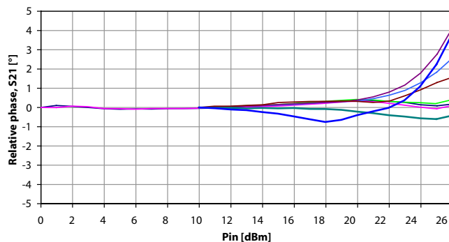
Relative Phase vs Input Power @ 10 GHz - Major States
