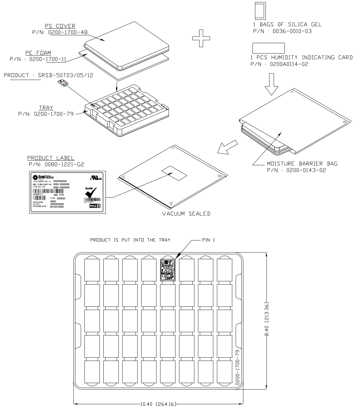
Figure 31. 0RSB-80T07LG / SRSB-80T07LG packaging information
