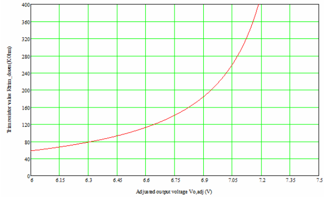
Figure 9. Trim down curve
