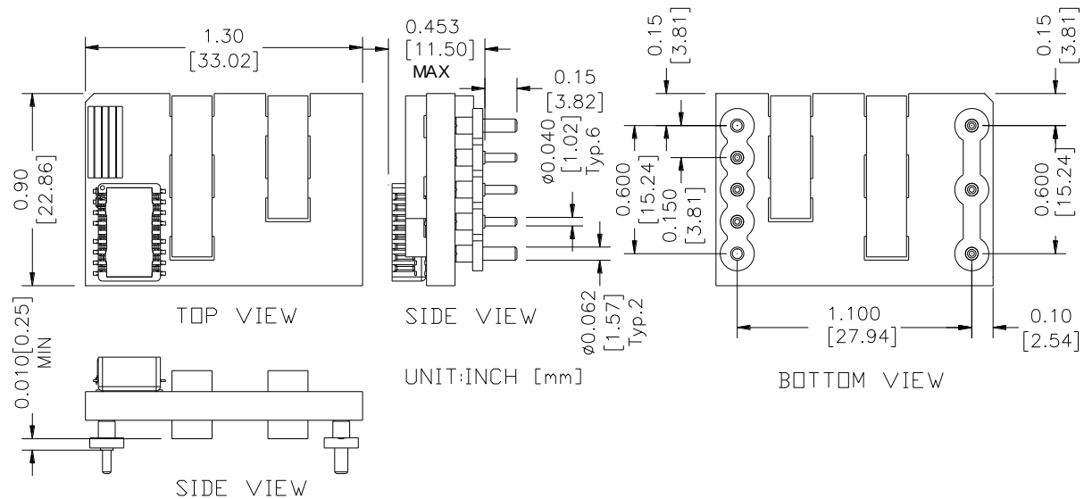
Figure 24. 0RSB-80T07L Outline
