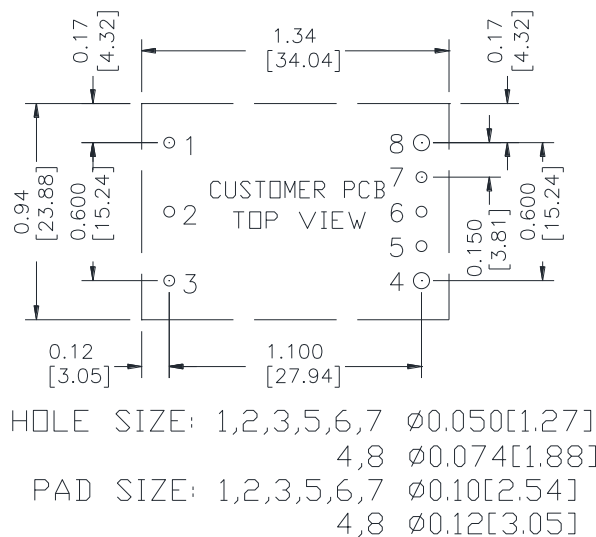
Figure 26. 0RSB-80T07L Recommended pad layout
