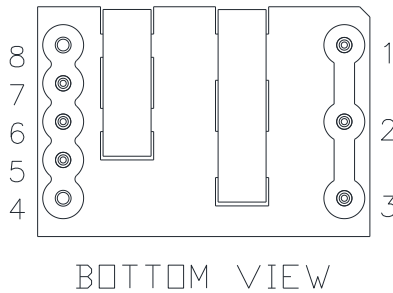
Figure 25. 0RSB-80T07L Pins
