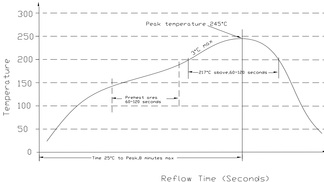
Figure 23. Soldering information
