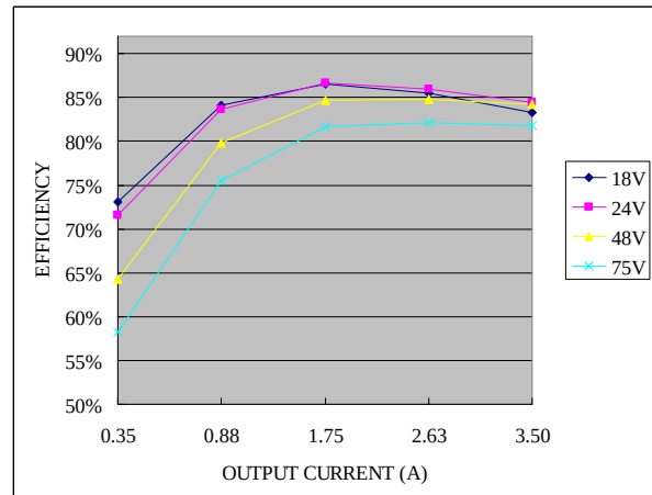
xRSB-40U12x
