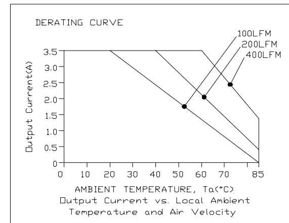
xRSB-40U12x
