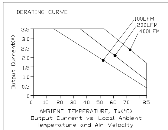
xRSB-40U12x
