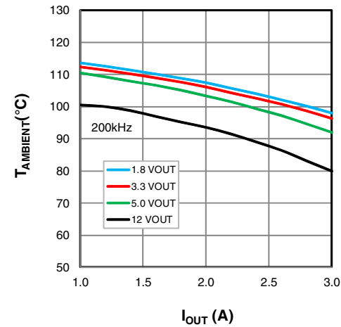
Figure 30: XR76203, V_{IN}=24\text{V}
