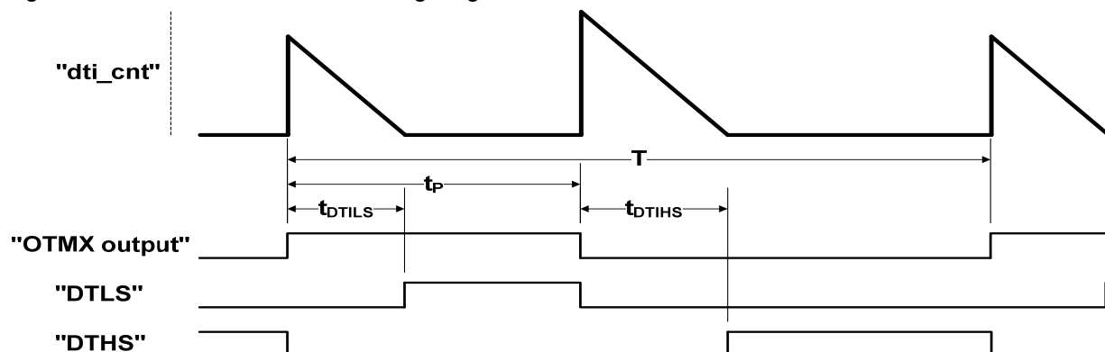
Figure 14-4. Dead-time Generator Timing Diagram
