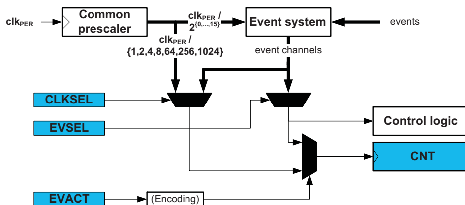
Figure 13-3. Clock and Event Selection
