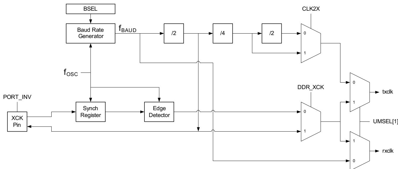
Figure 21-2. Clock Generation Logic Block Diagram
