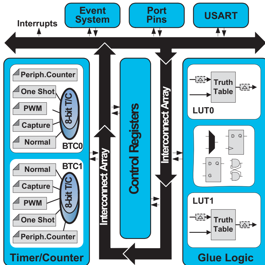
Figure 23-1. XCL Block Diagram and Closely Related Peripherals
