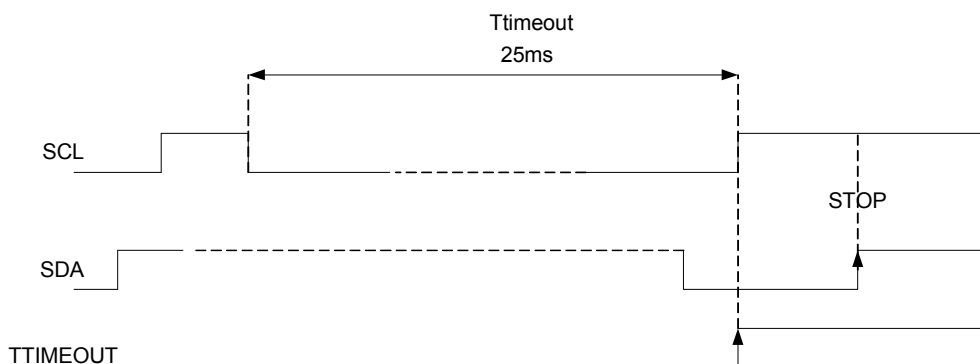
Figure 18-15.Timeout Condition
