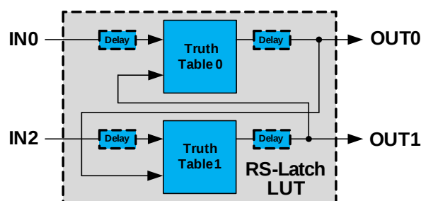
Figure 23-24. One RS-Latch LUT (RSLATCH)
