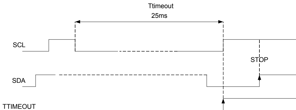
Figure 19-1. Timeout Condition
