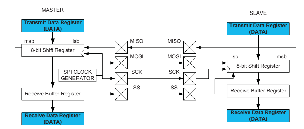
Figure 20-1. SPI Master-slave Interconnection
