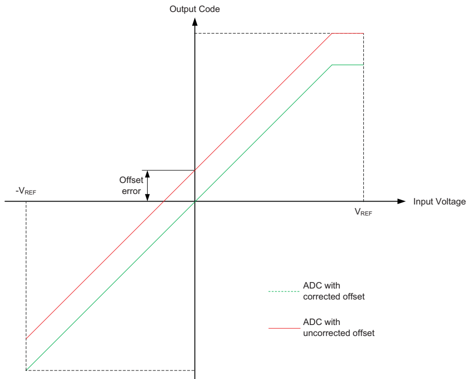
Figure 25-8. ADC Offset Error
