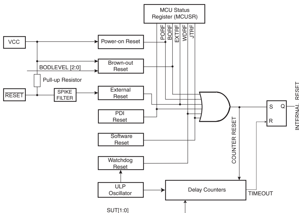
Figure 9-1. Reset System Overview
