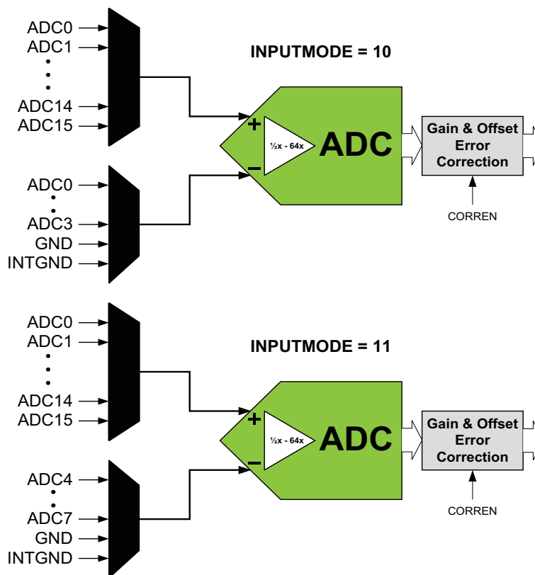
Figure 25-2. Differential Measurement
