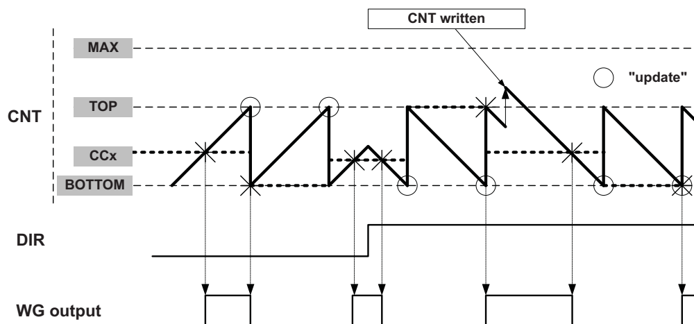
Figure 13-6. Normal Operation
