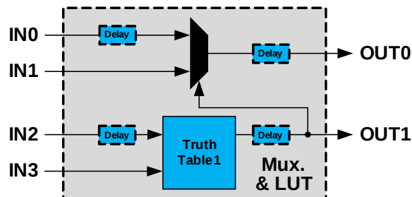
Figure 23-22. One 2-input Multiplexer Controlled by One 2-input LUT (MUX)
