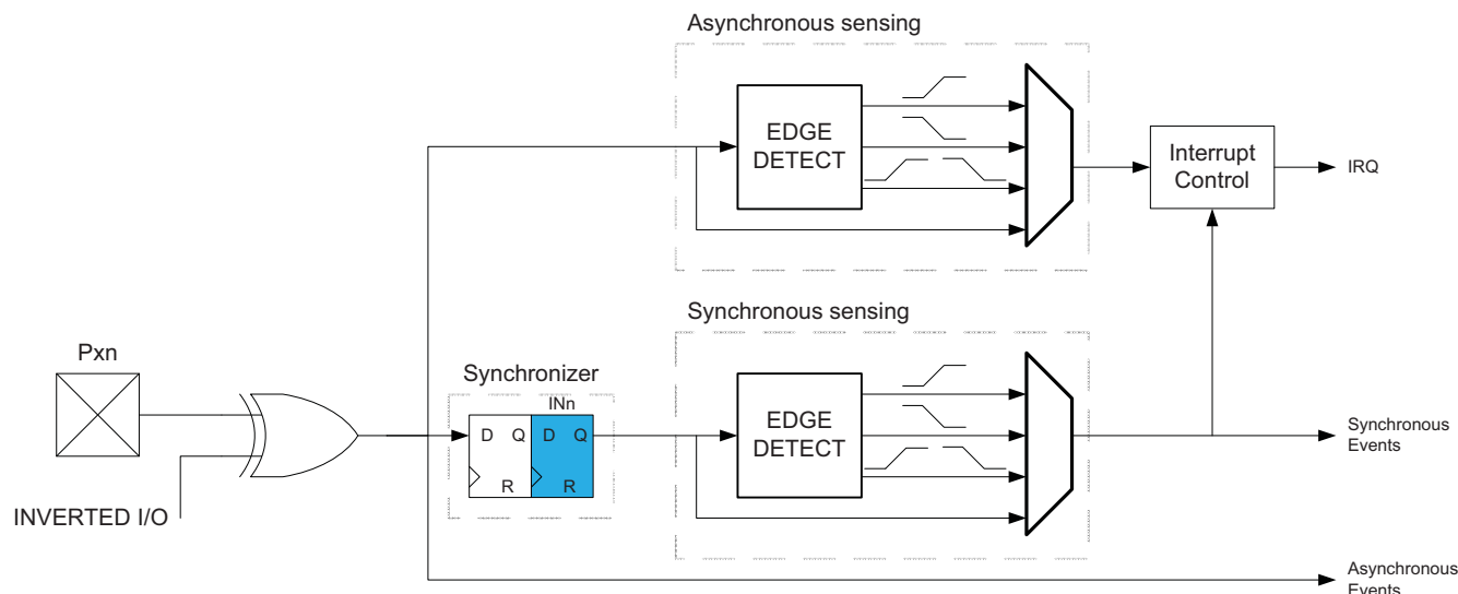
Figure 12-9. Input Sensing
