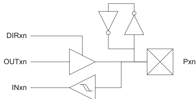
Figure 12-5. I/O Pin Configuration - Totem-pole with Bus-keeper
