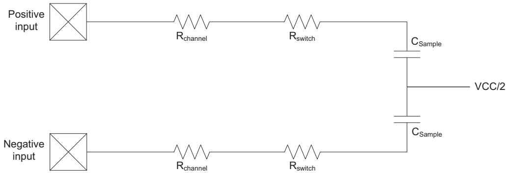
Figure 25-19.ADC Input for Differential Measurements and Differential Measurements with Gain
