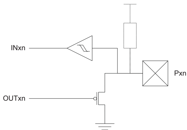
Figure 12-7. Output Configuration - Wired-AND with Optional Pull-up
