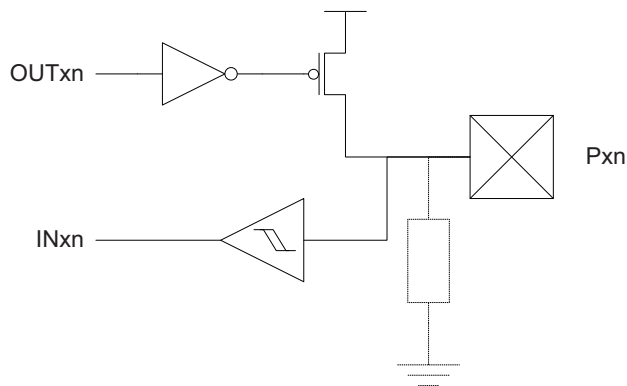
Figure 12-6. Output Configuration - Wired-OR with Optional Pull-down
