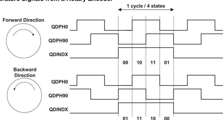
Figure 6-4. Quadrature Signals from a Rotary Encoder
