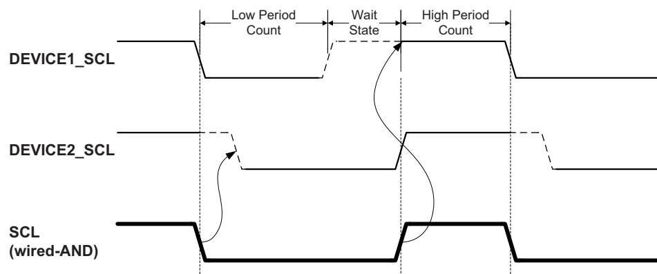
Figure 19-10. Clock Synchronization
