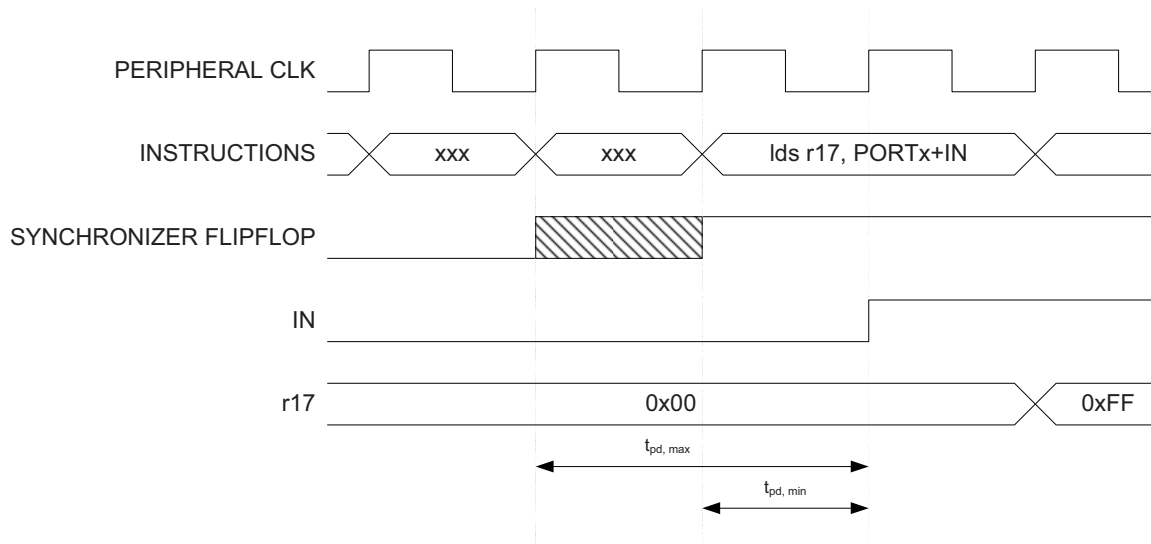
Figure 12-8. Synchronization when Reading a Pin Value
