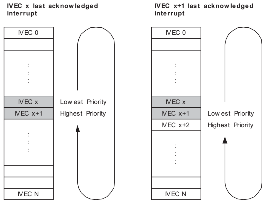
Figure 11-4. Round-robin Scheduling
