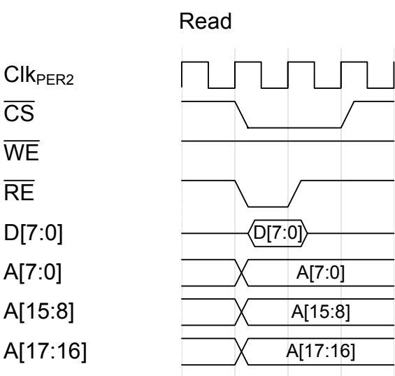
Figure 33-16. Read
