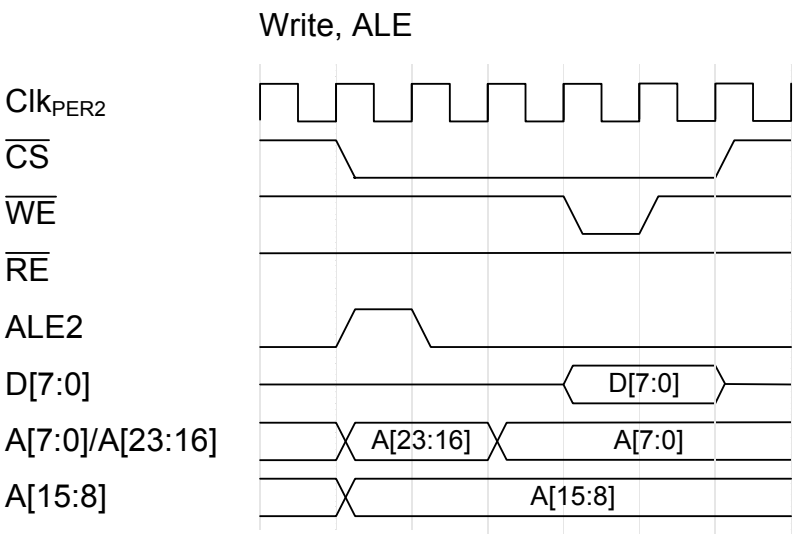
Figure 33-12. Write, ALE
