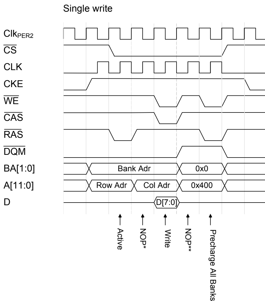
Figure 33-36. Single write
