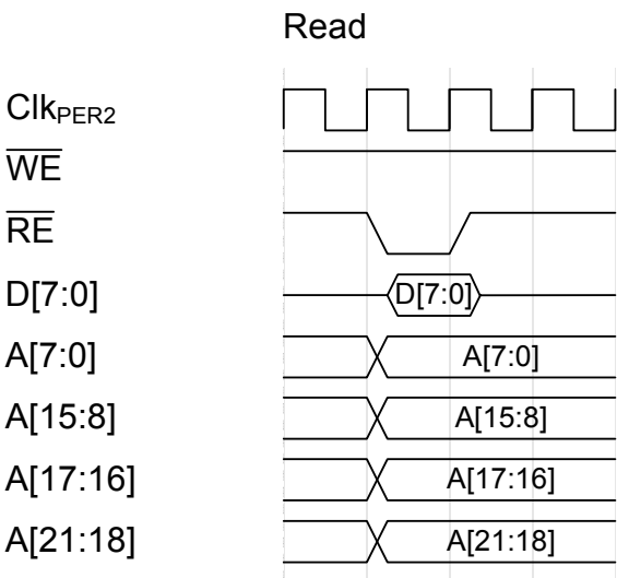
Figure 33-30.Read
