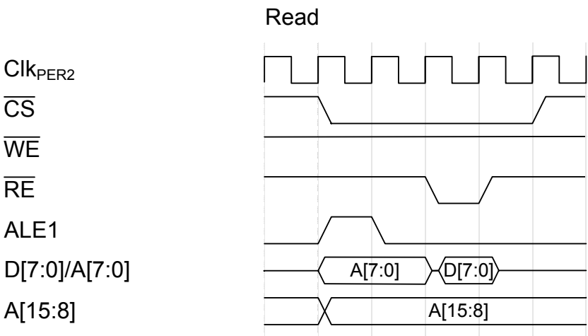
Figure 33-22. Read
