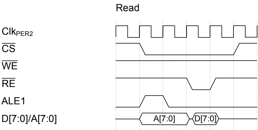
Figure 33-24. Read
