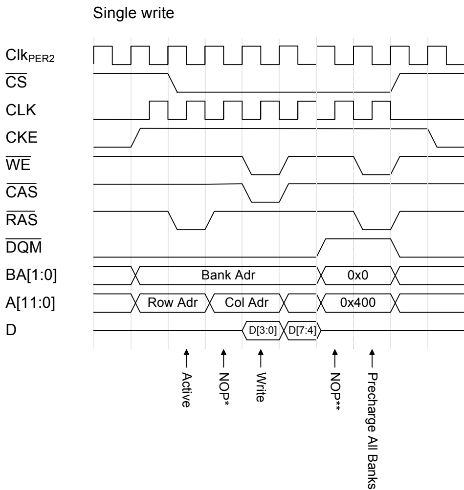
Figure 33-44. Single write
