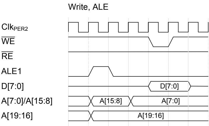
Figure 33-26. Write, ALE
