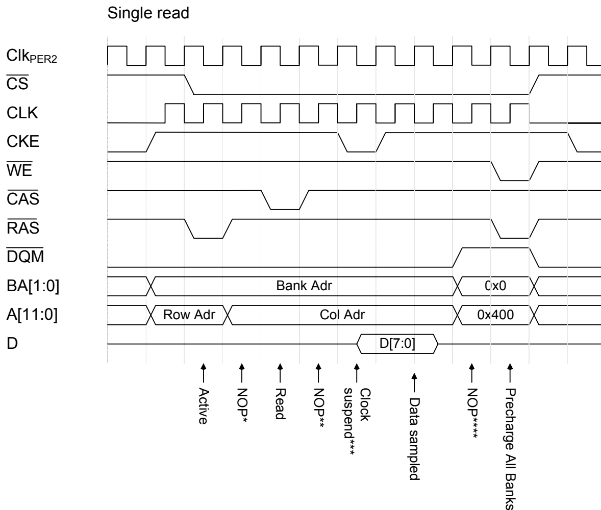
Figure 33-40. Single read
