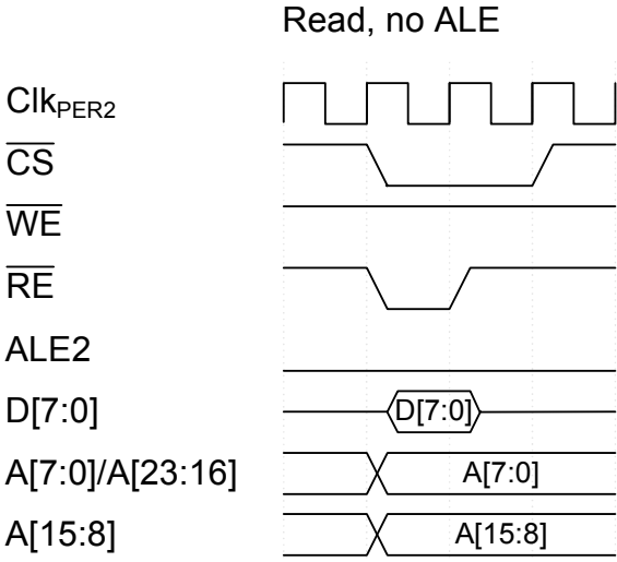
Figure 33-13.Read, no ALE
