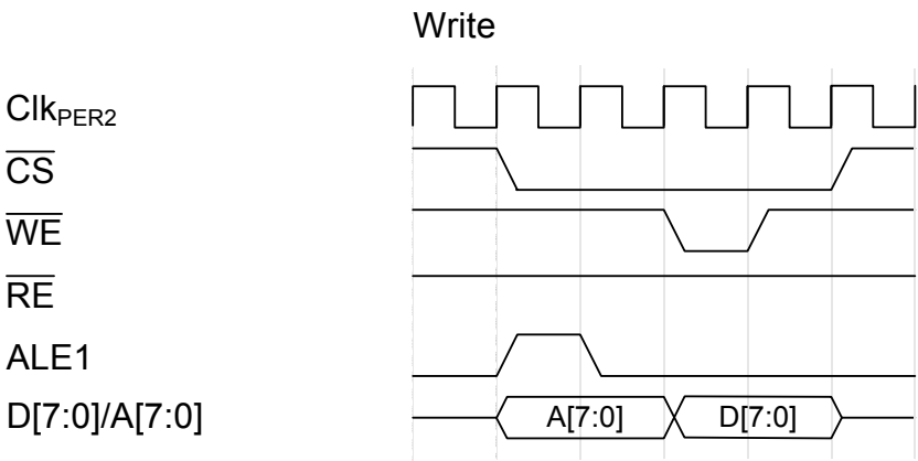
Figure 33-23. Write
