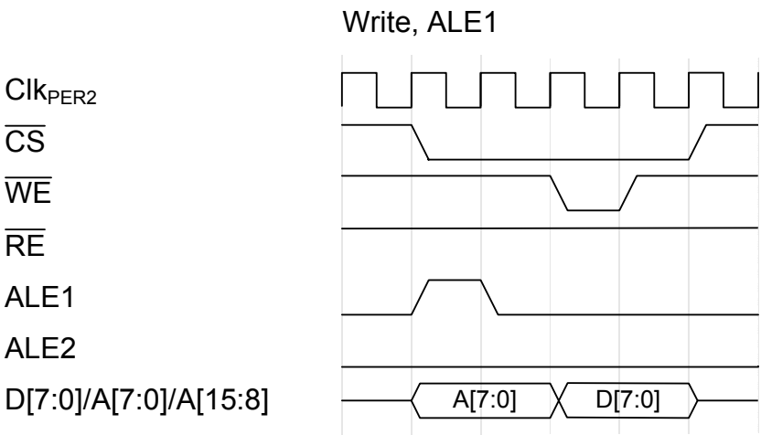
Figure 33-17. Write, ALE1
