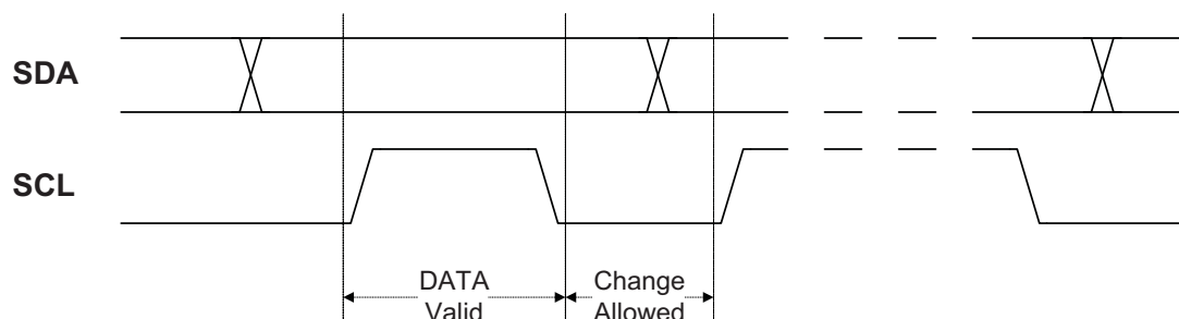
Figure 19-4. Data validity.
