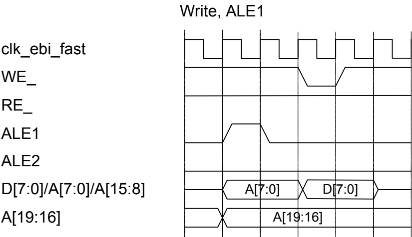
Figure 33-31. Write, ALE1
