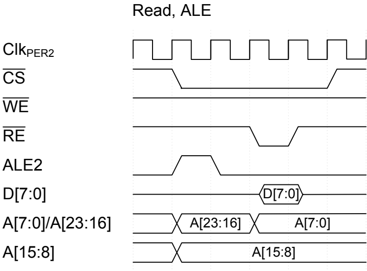
Figure 33-14.Read, ALE
