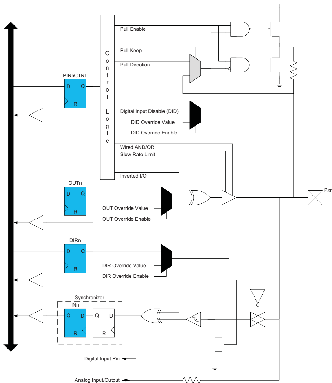
Figure 13-11. Port override signals and related logic.
