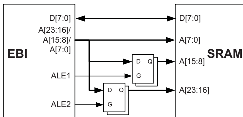
Figure 24-6. Multiplexed SRAM connection using ALE1 and ALE2.
