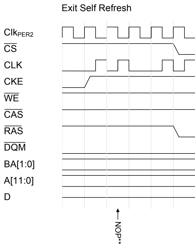
Figure 33-55.Exit Self Refresh
