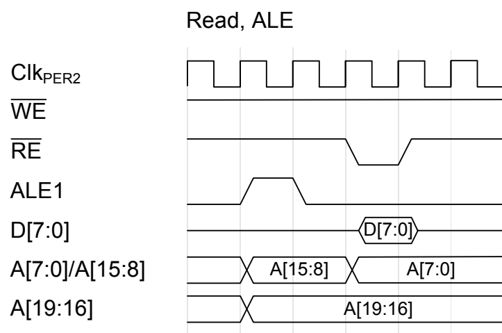
Figure 33-28. Read, ALE
