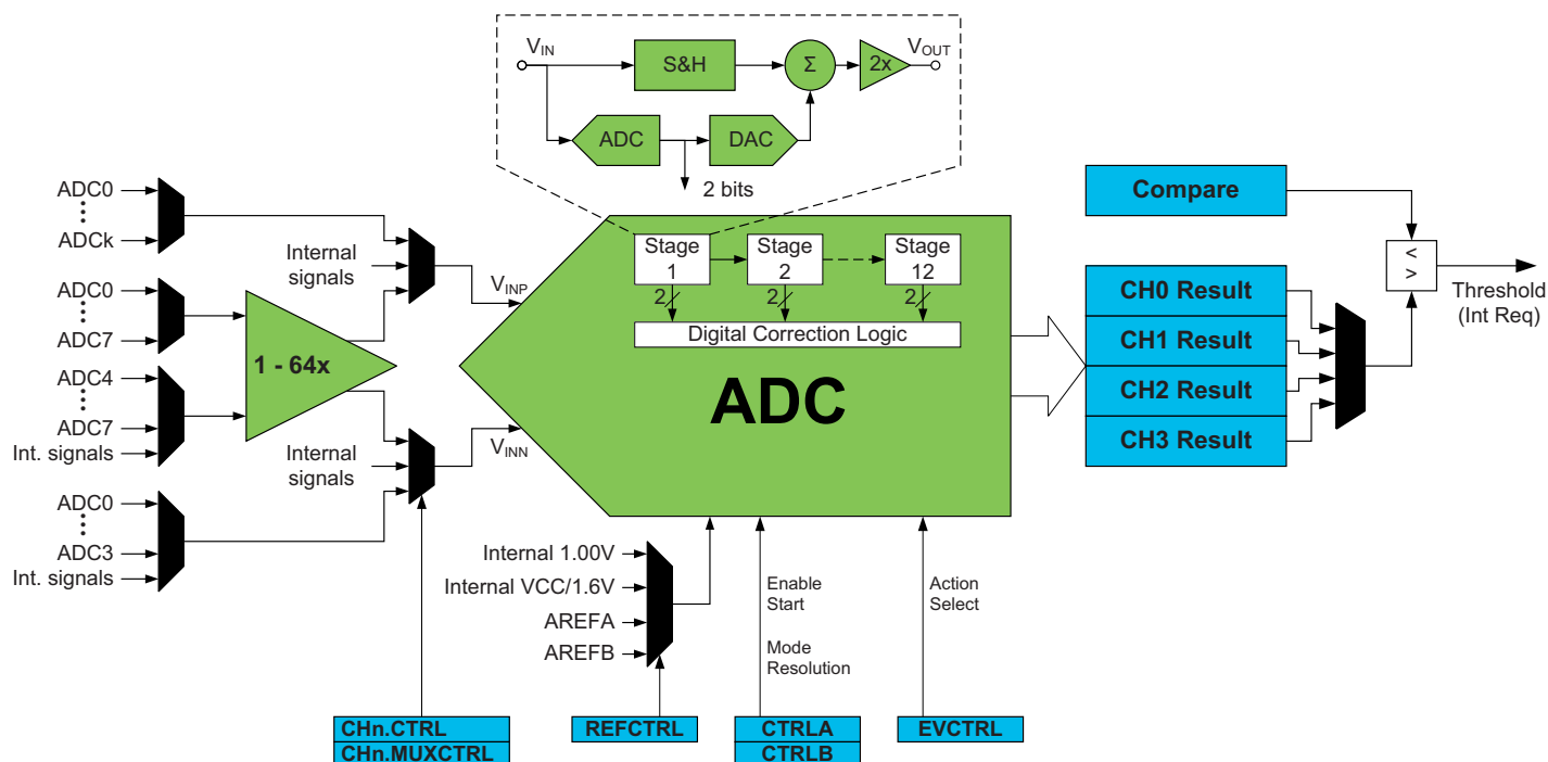
Figure 25-1. ADC overview.
