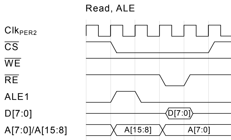
Figure 33-4. Read, ALE
