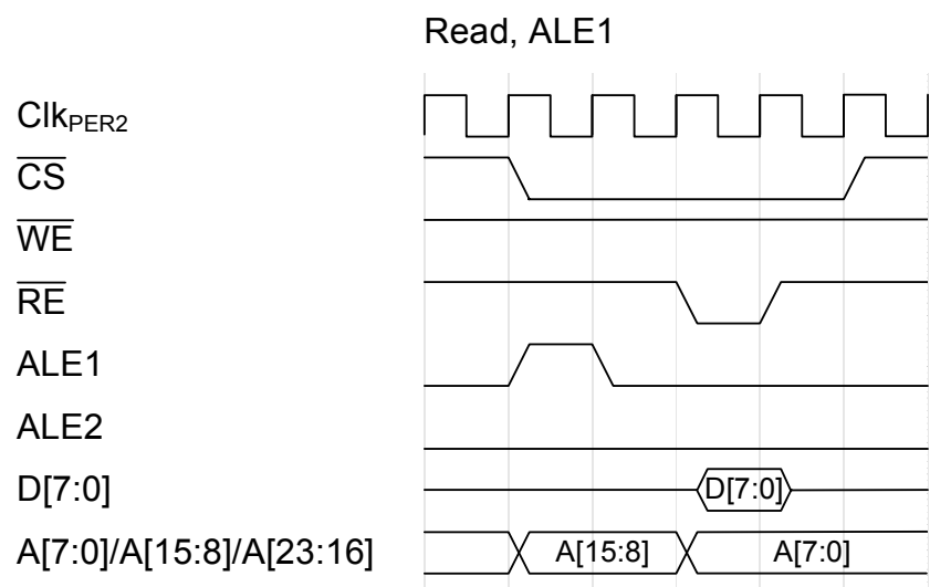
Figure 33-9. Read, ALE1
