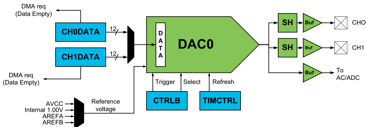
Figure 26-1. DAC overview.
