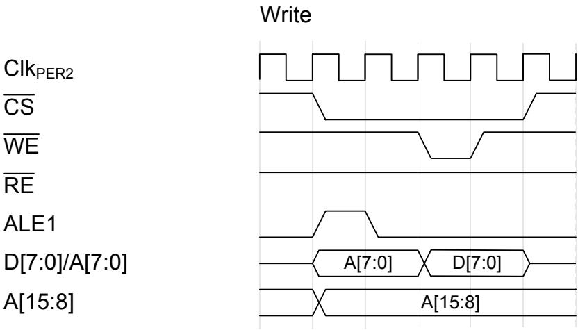
Figure 33-21. Write
