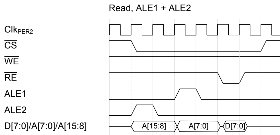
Figure 33-20.Read, ALE1 + ALE2
