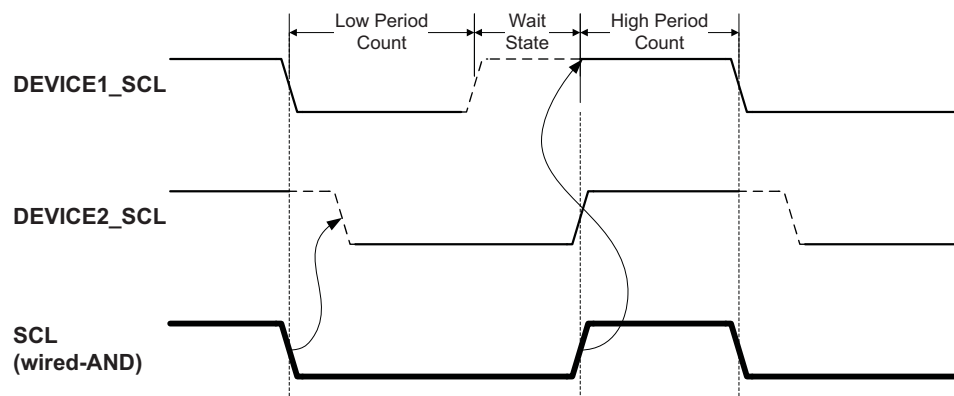
Figure 19-10. Clock synchronization.
