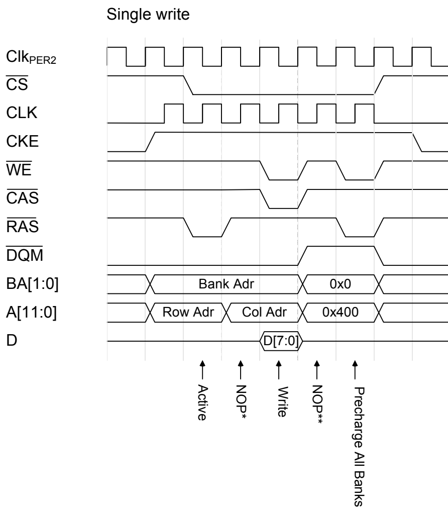
Figure 33-36. Single write
