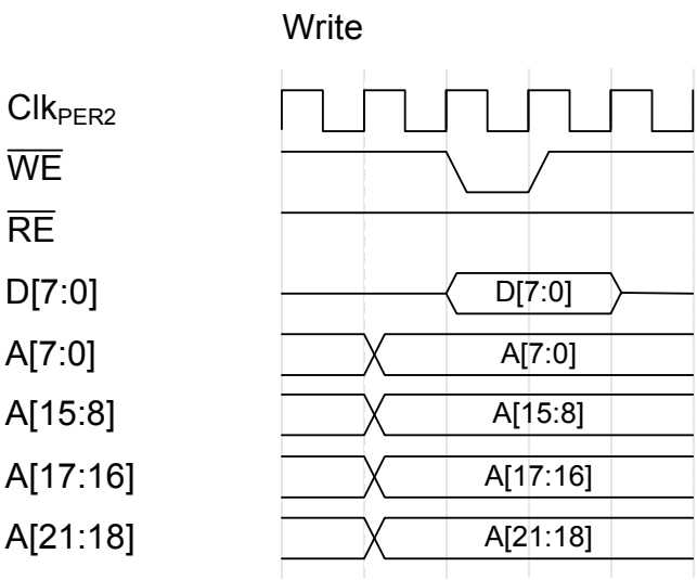
Figure 33-29.Write
