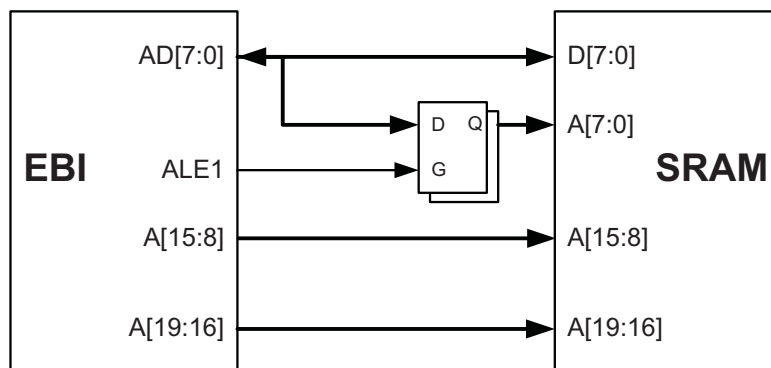
Figure 24-7. Multiplexed SRAM LPC connection using ALE1.
