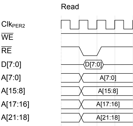
Figure 33-30.Read
