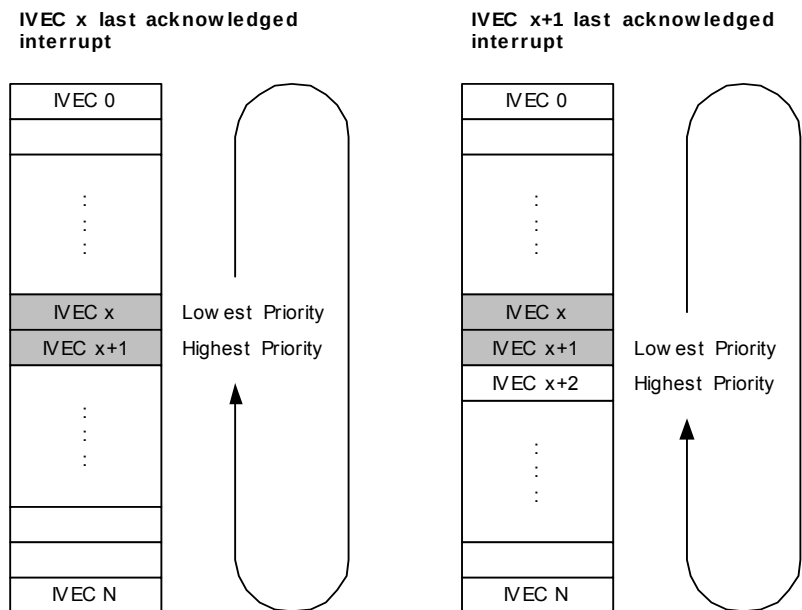
Figure 12-4. Round-robin scheduling.
