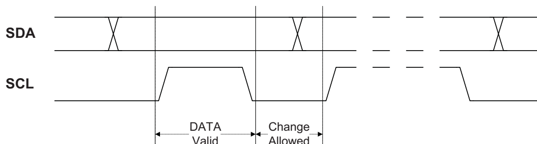
Figure 19-4. Data validity.
