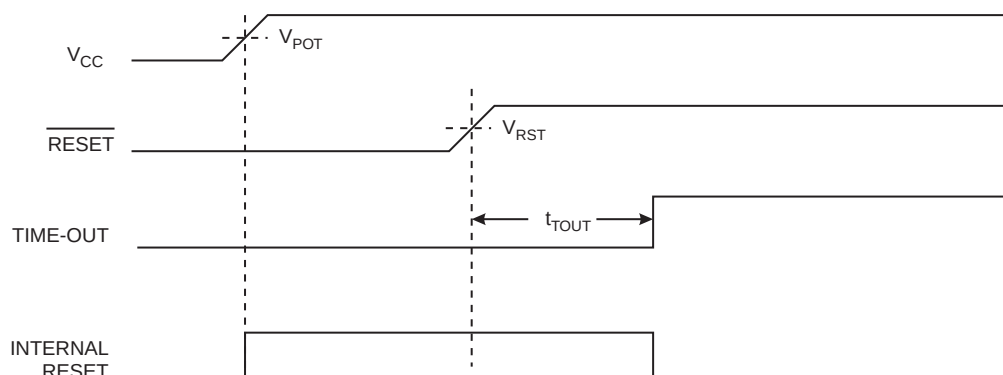
Figure 9-3. MCU startup, RESET extended externally,
