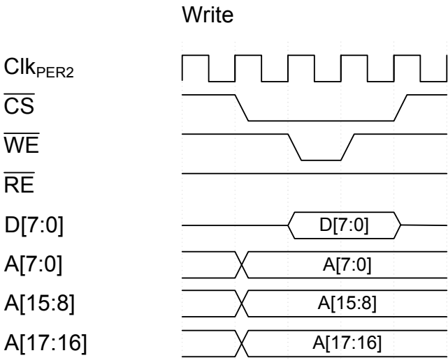
Figure 33-15. Write
