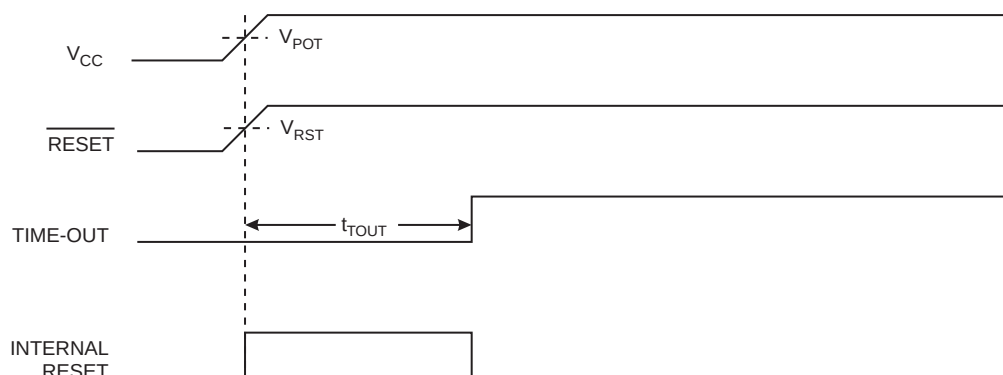
Figure 9-2. MCU startup, RESET tied to V_{CC} .
