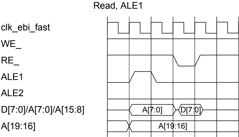
Figure 33-33.Read, ALE1
