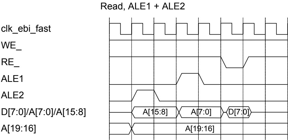
Figure 33-34.Read, ALE1 + ALE2
