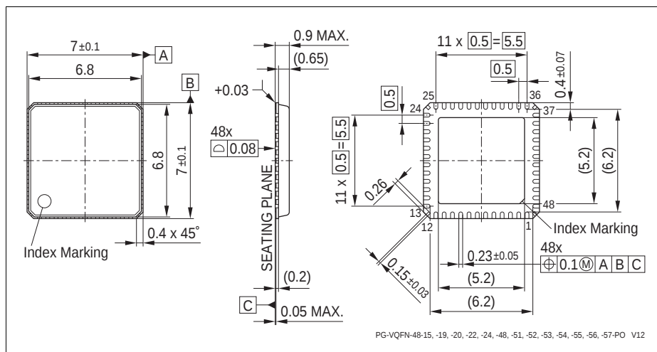
Figure 38 PG-VQFN-48-53 (Plastic Green Very Thin Profile Flat Non Leaded Package)
