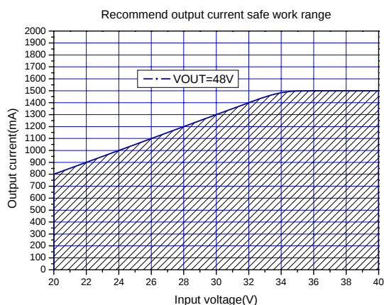
Figure8.Max output current(VOUT=48V)
