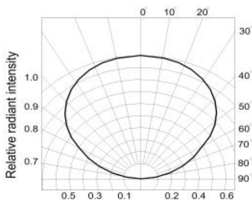
Fig. 6 Radiation diagram
