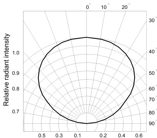
Fig.6 Radiation diagram
