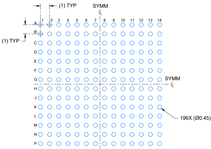
LAND PATTERN EXAMPLE SCALE: 5X
