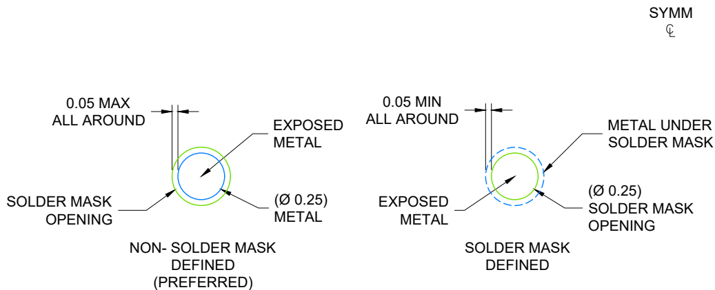
SOLDER MASK DETAILS NOT TO SCALE
