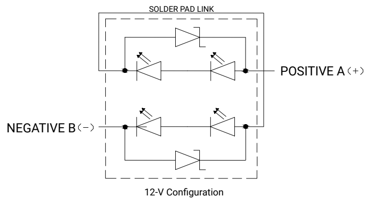
12-V Configuration
