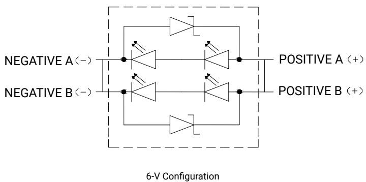
6-V Configuration
