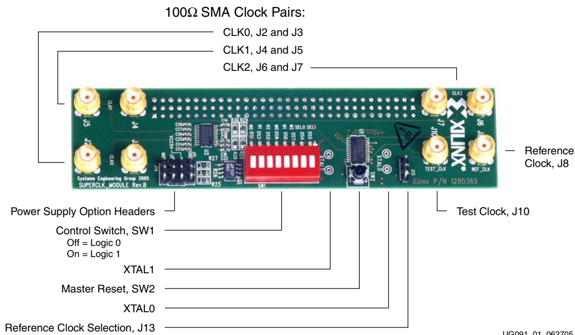
Figure 1: SuperClock Module, Front View
