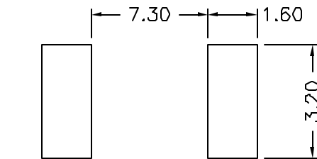
(SUGGESTED MOUNTING PAD)
